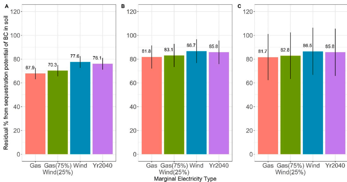
Fig. 4. Biochar soil carbon sequestration efficiency: the remaining carbon capture potential of biochar in soils of after accounting for all the processes, in percent. Section A, B and C represent the production of 100%, 50% and 25% of the maximum biochar production. The remaining residues in section B and C are treated in a CHP similarly to the baseline. The error bars are \pm 1 SD.
