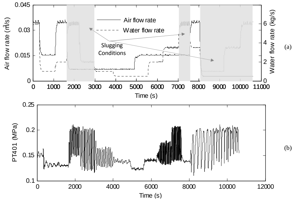
Fig. 8: Measured flow rates (a) and bottom riser pressure PT401 (b) for data set 5.2
