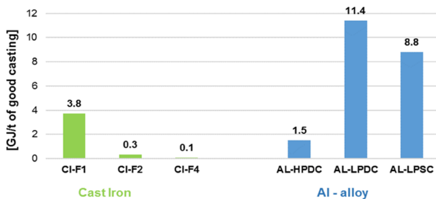
Figure 10: Miscellaneous energy monitoring at the foundries interviewed.
