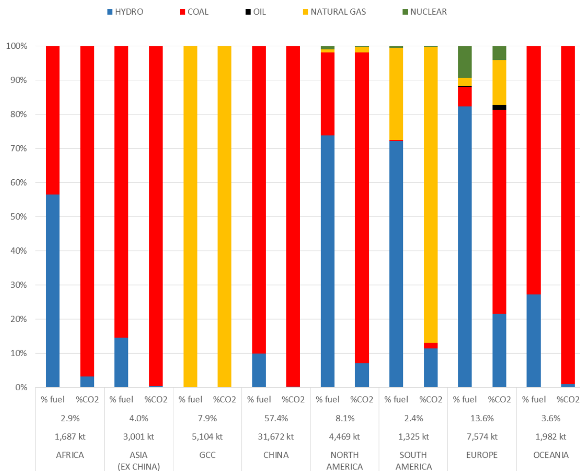
% of world and reported tonnage (kt) of aluminium production by region
