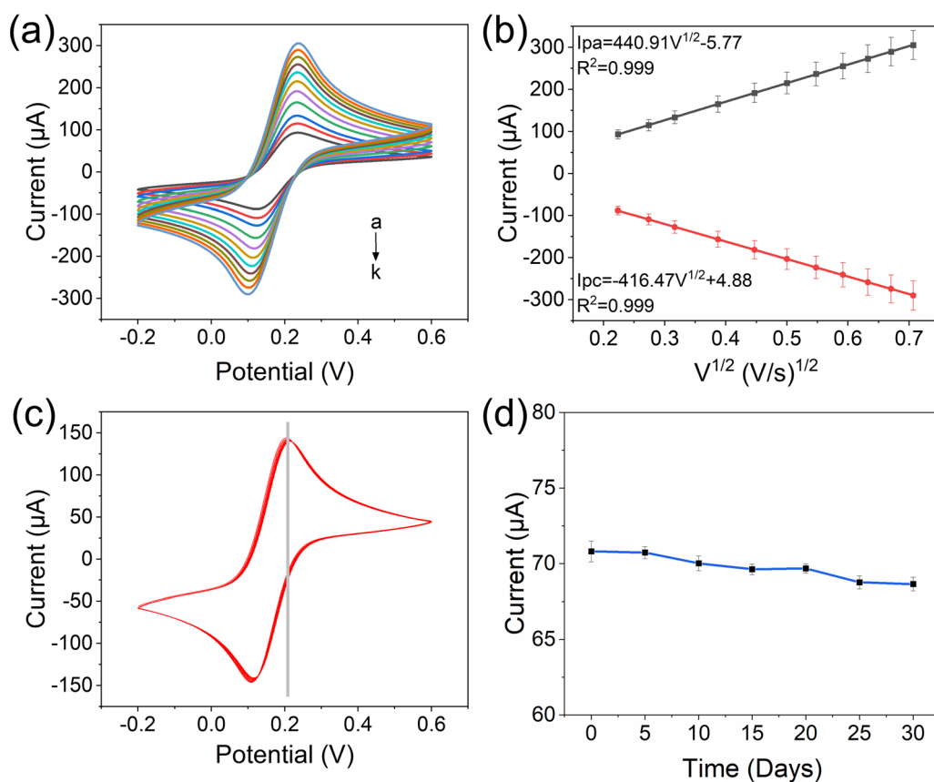
Figure 3 Electrochemical performance of GF-based electrode in 5 mM K 3 [Fe(CN) 6 ]/K 4 [Fe(CN) 6 ] and 0.1 M KCl. (a) Cyclic voltammetry measurements conducted at different scan rates (a-k: 0.05, 0.75, 0.1, 0.15, 0.2, 0.25, 0.3, 0.35, 0.4, 0.45 and 0.5 V s -1 ). (b) The peak current plotted as a function of the square root of the scan rate with the fitted linear regression curves. Black and red dots indicate anodic and cathodic peak currents, respectively. (c) 10 cycles of CV recorded at scan rate of 0.1 V s -1 . (d) Stability test of the GF-based electrode with different times. Error bars were obtained from 3 successive DPV measurements with the same device.
