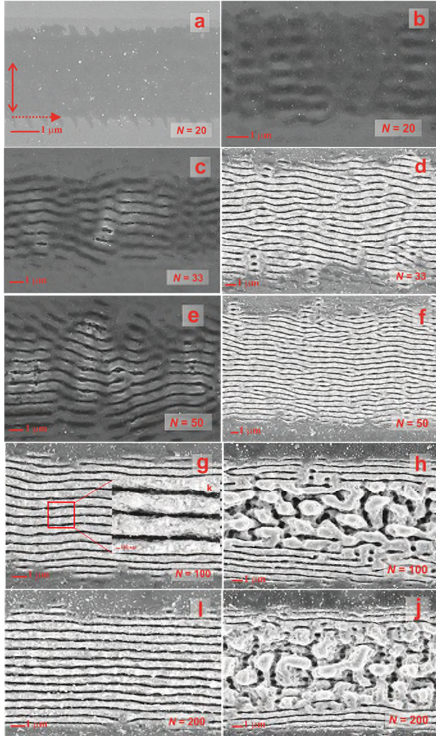
Figure 2. FESEM images of Si surface in air after irradiation with fs laser pulses. Figures (a), (c), (e), (g) and (i) are written with laser fluence of 0.3 \text{ Jcm}^{-2} ; (b), (d), (f), (h) and (j) are written with laser fluence of 0.42 \text{ Jcm}^{-2} . Figure 2(k) shows magnified FESEM image of laser induced periodic features of figure 2(g). Applied number of laser pulses is labeled on the images, laser polarization and writing directions are indicated by the solid and dotted arrows, respectively in figure 2(a).
