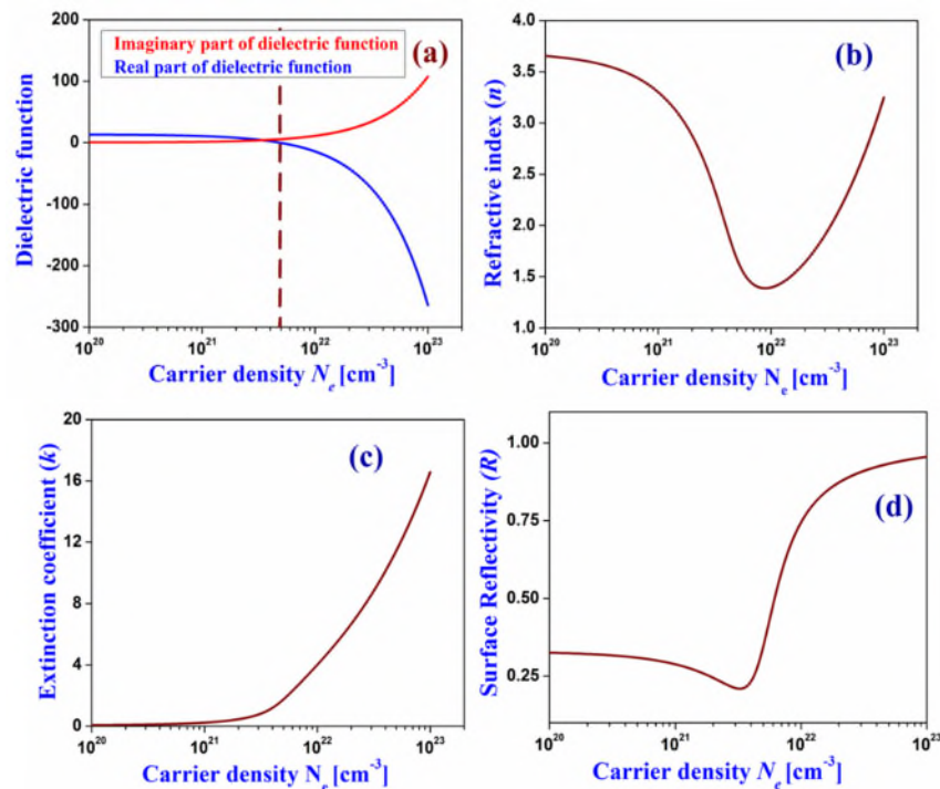
Figure 5. Optical properties of fs laser irradiated single-crystalline silicon as a function of the excited carrier densities N_e for the irradiation wavelength of 800 nm. (a) Real and imaginary parts of dielectric function, dotted line in the plots indicates the critical carrier density above which the Si surface exhibits a sharp transition from semiconductor to metallic nature, (b) Refractive index n^*(N_e) , (c) Extinction coefficient k^*(N_e) and (d) Surface reflectivity R^*(N_e) .
