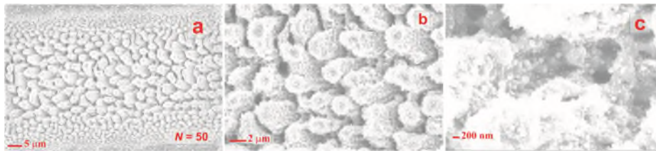
Figure 3. (a) FESEM micrographs of Si surface in air after irradiation with laser fluence of 0.65 \text{Jcm}^{-2} . (b) and (c) represents high resolution images of (a).
