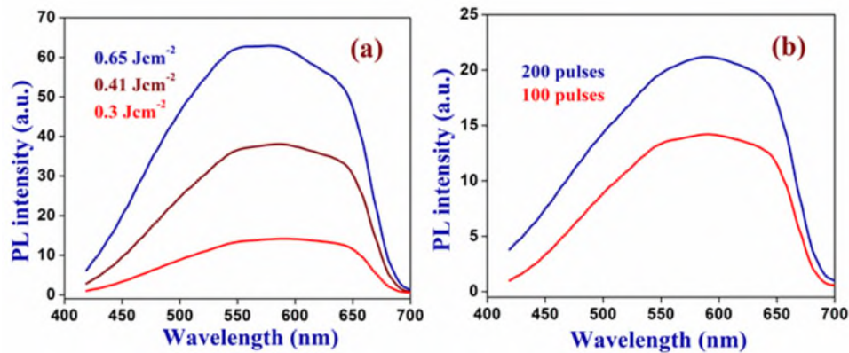
Figure 8: Photoluminescence spectrum of fs laser irradiated silicon surface under the excitation of 365 nm wavelength. (a) Function of laser fluence ( F ) used to irradiate the silicon surface and (b) function of laser pulses ( N ) with fluence F = 0.3\text{ Jcm}^{-2} used to irradiate the silicon surface
