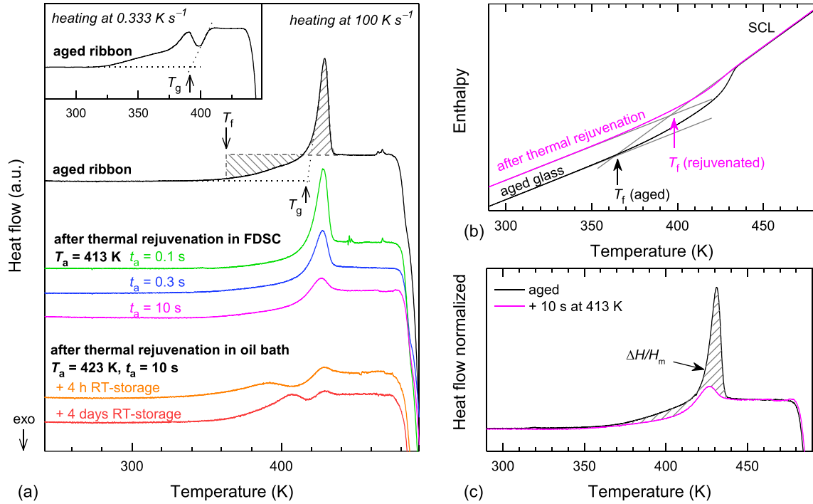
Fig. 1. (a) Example heat-flow trace measured at 100 K s -1 of the aged Au-based MG ribbon in its initial state, after thermal rejuvenation in FDSC (at 413 K for various times t_a , followed by quenching at 100 K s -1 ) and after thermal rejuvenation in oil and water quenching, followed by RT-storage for approximately 4 h and 4 days. The inset shows the heat-flow trace of the aged ribbon on heating at 0.33 K min -1 by conventional DSC. An example of the determination of the fictive temperature T_f via the equal-area construction is shown in the case of the aged sample by the hatched areas. (b) Enthalpy-temperature plot of the aged ribbon and after thermal rejuvenation (based on measured data [18]). The intersection of the supercooled liquid (SCL) enthalpy line with that of the glass corresponds to T_f . (c) The normalized increase in enthalpy \Delta H/H_m determined as the area (hatched) between the curves of the aged ribbon in its initial state and after thermal rejuvenation (10 s at 413 K, cooled at 100 K s -1 ), after normalization of the curves to their heat of melting H_m .
