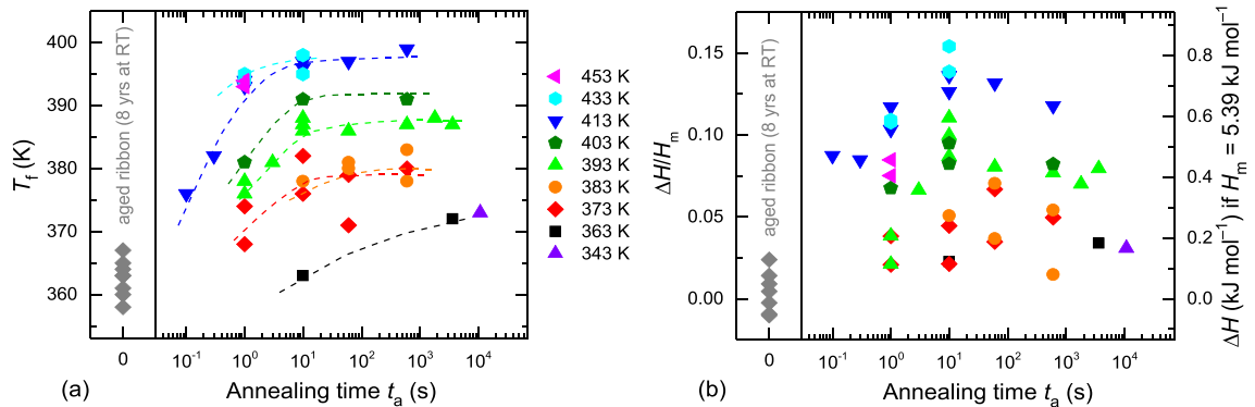
Fig. 2. The increase (a) in fictive temperature T_f and (b) in enthalpy \Delta H/H_m of the 8-yr-aged ribbon after thermal rejuvenation at different temperatures and times, followed by cooling at 100 K s -1 by FDSC. The dashed lines in (a) are a guide for the eyes.
