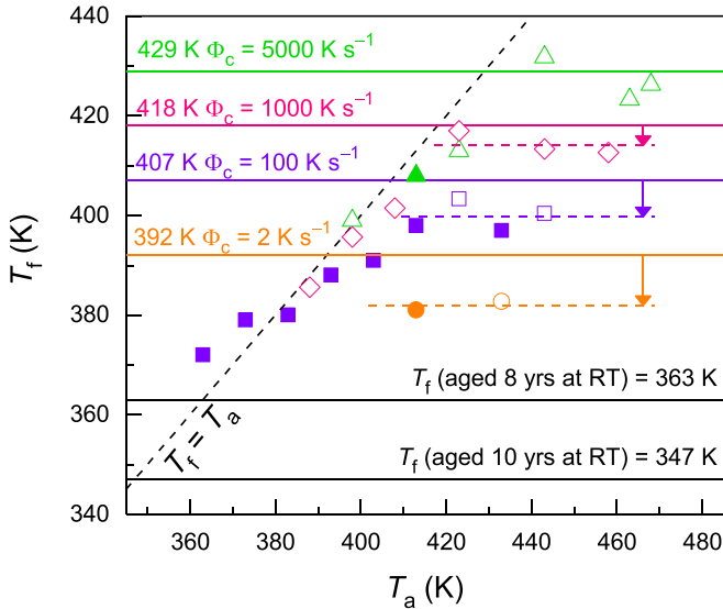
Fig. 3. Estimation of saturation values of T_f as a function of the rejuvenation temperature T_a . The cooling rate \Phi_c after annealing is 2 \text{ K s}^{-1} (orange circles), 100 \text{ K s}^{-1} (violet squares), 1000 \text{ K s}^{-1} (pink diamonds) and 5000 \text{ K s}^{-1} (green triangles). The full data points were measured on the 8-yr-aged ribbon and the open points on the 10-yr-aged ribbon. The solid lines at 392 K, 407 K, 418 K and 429 K correspond to the expected T_f for a glass formed upon quenching the melt at 2 \text{ K s}^{-1} , 100 \text{ K s}^{-1} , 1000 \text{ K s}^{-1} , and 5000 \text{ K s}^{-1} , respectively, according to Monnier et al. [17]. (For interpretation of the references to colour in this figure legend, the reader is referred to the web version of this article.)
