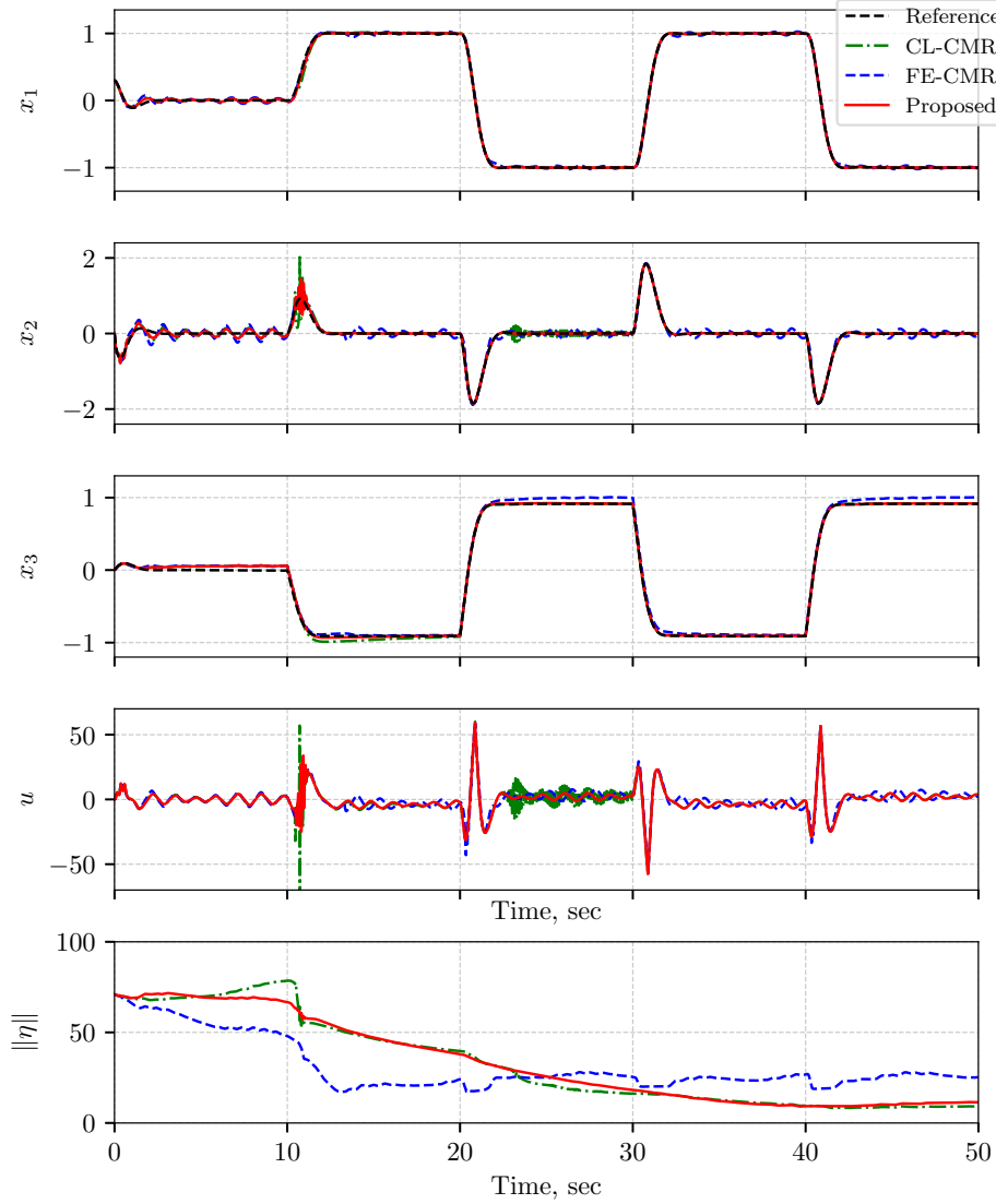
Fig. 1. The state, control input, and tracking error responses.
