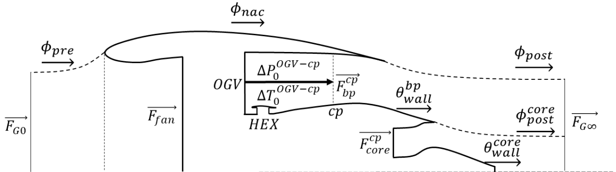
Figure 3 Thrust and Drag accounting for engine with HEX system installed within the bypass duct.
