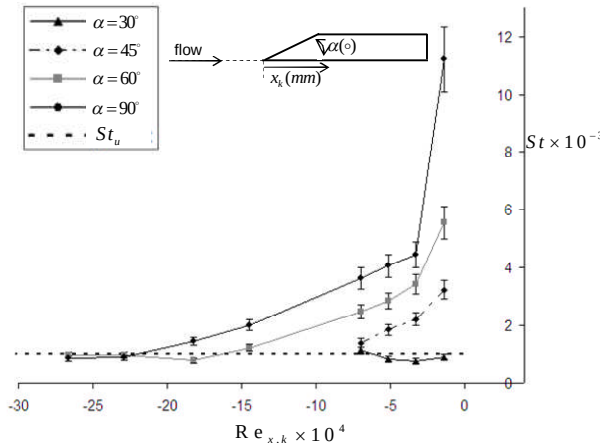
Fig. 8 Heat flux along the centreline ( y_{cl}=0\text{mm} ) as a function of protuberance deflection angle. Turbulent, M_\infty=8.2 , Re_\infty/m=9.35 \times 10^6 , \alpha=30^\circ to \alpha=90^\circ .
