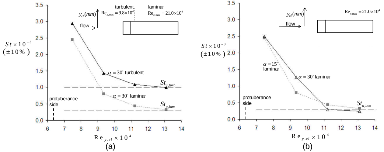
Fig. 12 Spanwise distribution of heat transfer and peak axial locations to the side of \alpha=30^\circ protuberance for laminar and turbulent conditions (a) and to the side of \alpha=15^\circ and \alpha=30^\circ models for laminar conditions (b).
