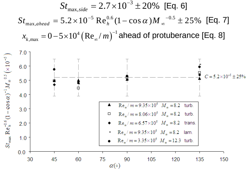
Fig. 19 Correlation of the whole hot-spot experimental dataset showing uncertainty of \pm 25\% .
