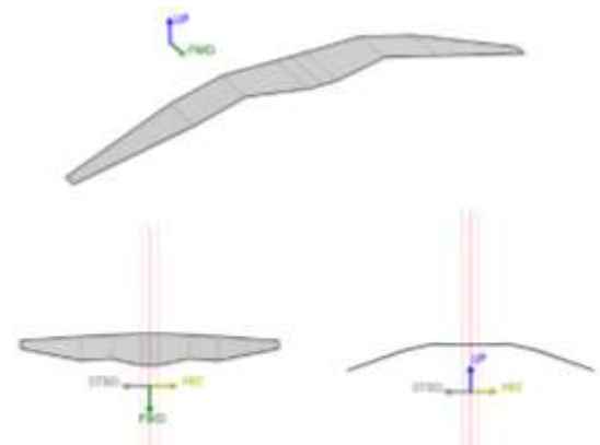
Fig. 3: Albatross bioinspired wing
