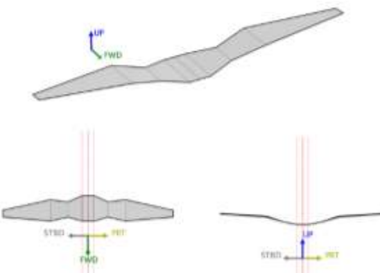
Fig. 4: Frigatebird bioinspired wing
