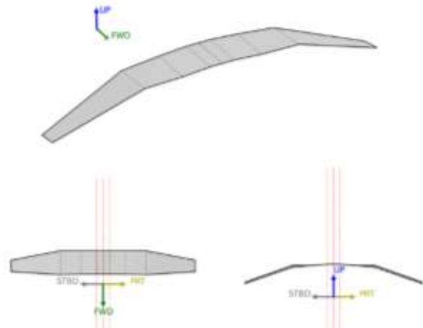
Fig. 5: Pelican bioinspired wing
