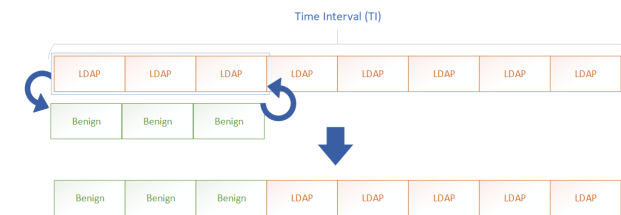
FIGURE 19. Sequence traffic adjustment during and after splice.
