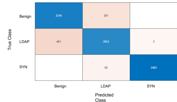
FIGURE 29. Confusion matrix for CIC 2019 training set utilising a randomised subset.
