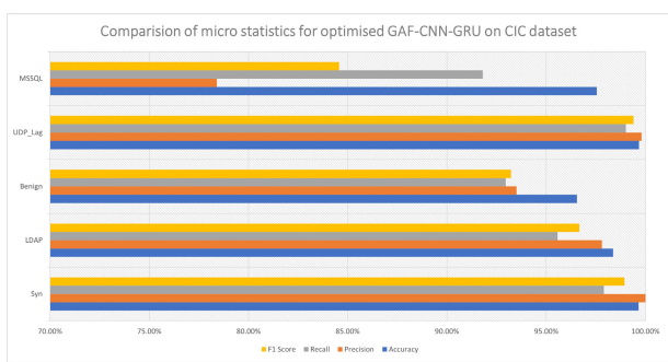
FIGURE 32. Micro statistics of accuracy, precision, recall and f1 Score across CIC Dataset Classes.
