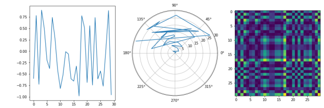
FIGURE 21. One-dimensional time series converted to two-dimensional images in polar coordinate system.
