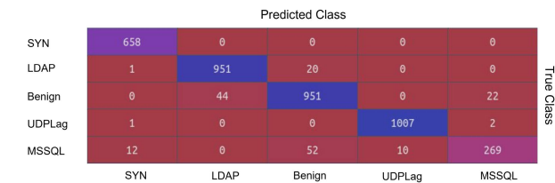
FIGURE 31. Confusion matrix for CIC 2019 validation set using the optimised feature subset.
