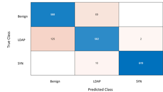
FIGURE 30. Confusion matrix for CIC 2019 validation set using a randomised subset.
