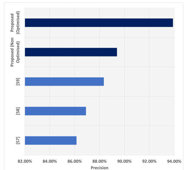
FIGURE 39. Precision comparison of mf-CNNGAF and other models in multi-class classification on the CIC dataset.
