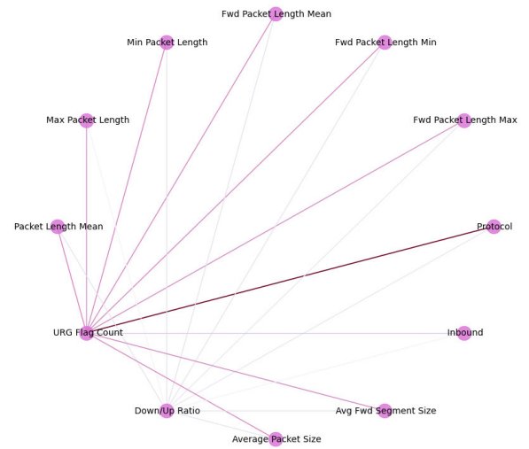
FIGURE 12. Graphical representation of weighted negative feature correlations.
