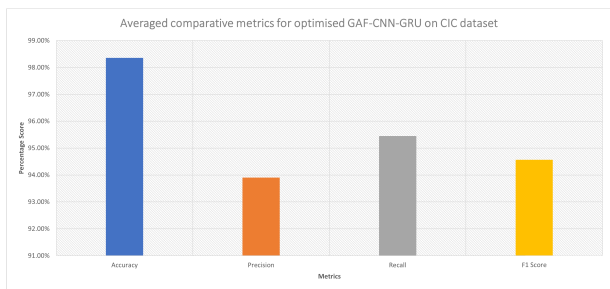
FIGURE 33. Averaged statistics of accuracy, precision, recall and f1 Score across optimised CIC Dataset Classes.
