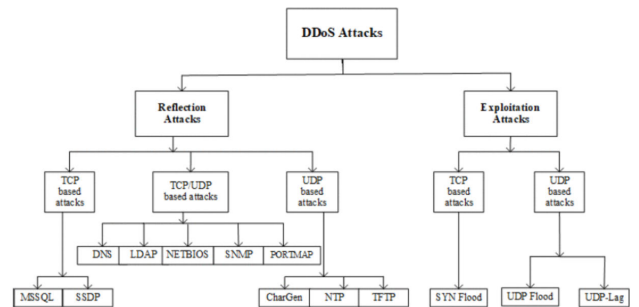
FIGURE 8. CIC 2019 Dataset Taxonomy [23].
