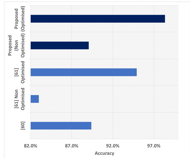
FIGURE 42. Accuracy of mf-CNNGAF compared to other CNN driven models in multi-class classification on the CIC dataset.
