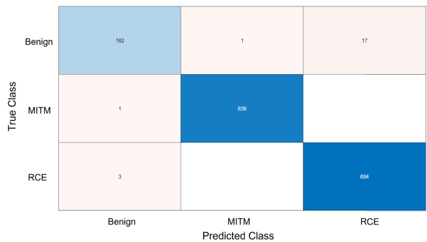
FIGURE 34. Validation confusion matrix when applied to Cranfield Cyber Security Dataset.
