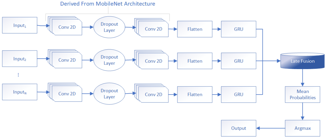
FIGURE 25. CNN-GRU Architecture.
