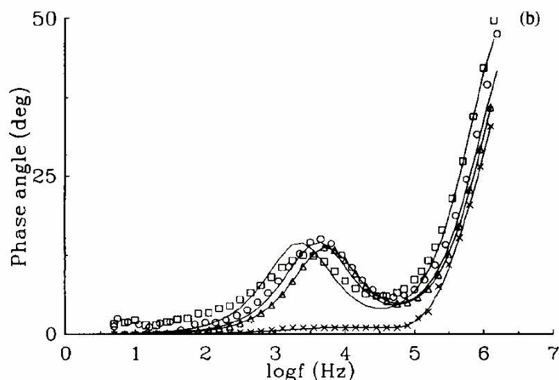
Fig. 4. Bode plots (a) \log|Z| and (b) phase angle, for different types of coated steel specimens exposed to 3.5% NaCl solution for 4 h: \times , pure epoxy; \triangle , 7.5%; \circ , 15%; \square , 30% wt./wt. iron powder.
