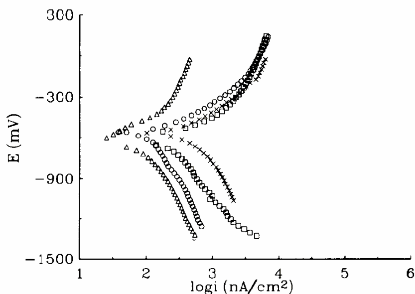
Fig. 2. Potentiodynamic polarization plots of different types of coated steel specimens exposed to 3.5% NaCl solution for 4 h: \times , pure epoxy; \Delta , 7.5%; \circ , 15%; \square , 30% wt./wt. iron powder.
