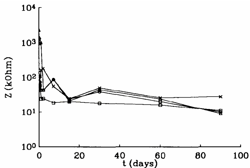
Fig. 6. Impedance time dependence for different types of coated steel specimens: X, pure epoxy; \Delta , 7.5%; \circ , 15%; \square , 30% wt./wt. iron powder.
