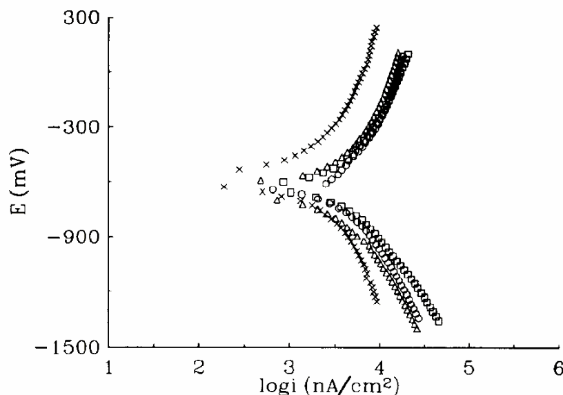
Fig. 3. Potentiodynamic polarization plots for different types of coated steel specimens exposed to 3.5% NaCl solution for 90 days: \times , pure epoxy; \Delta , 7.5%; \circ , 15%; \square , 30% wt./wt. iron powder.
