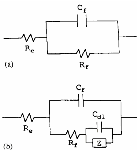
Fig. 7. Electrical equivalent circuit generally accepted for a coated metal/solution interface without diffusion: (a) barrier coatings; (b) non-barrier coating.
