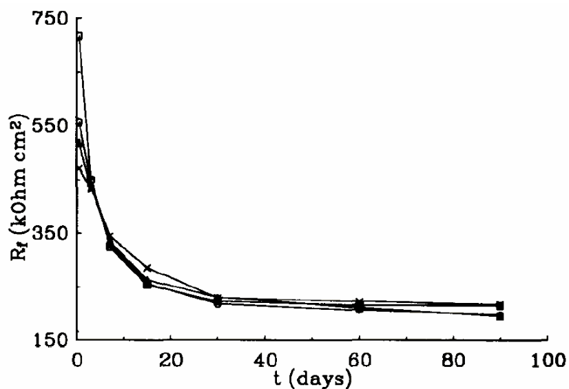
Fig. 8. Change of coating resistance R_f with exposure time for different types of coated steel specimens obtained by ZSIM: X, pure epoxy; \Delta , 7.5%; \circ , 15%; \square , 30% wt./wt. iron powder.
