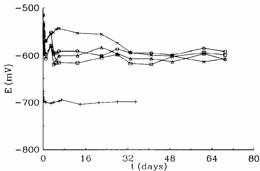
Fig. 1. Time dependence of corrosion potential for different types of coated and uncoated steel specimens: +, bare steel; X, pure epoxy; \triangle , 7.5%; \circ , 15%; \square , 30% wt./wt. iron powder.
