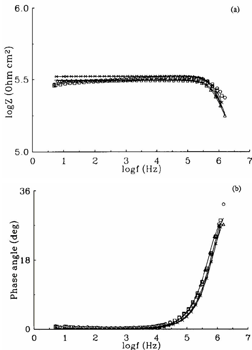
Fig. 5. Bode plots (a) \log|Z| and (b) phase angle, for different types of coated steel specimens exposed to 3.5% NaCl solution for 90 days: \times , pure epoxy; \triangle , 7.5%; \circ , 15%; \square , 30% wt./wt. iron powder.
