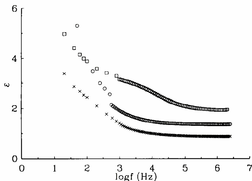
Fig. 10. Dielectric permittivity vs. frequency for different types of coated steel specimens after one day of immersion: \times , pure epoxy; \circ , 15%; \square , 30% wt./wt. iron powder.
