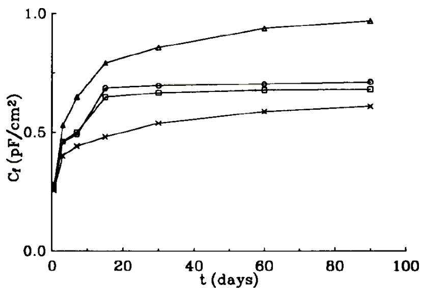
Fig. 9. Change of coating capacitance C_f with exposure time for different types of coated steel specimens obtained by ZSIM: X, pure epoxy; \Delta , 7.5%; \circ , 15%; \square , 30% wt./wt. iron powder.
