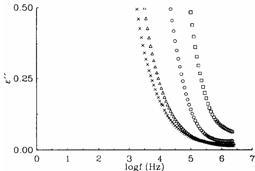
Fig. 12. Dielectric loss vs. frequency for the coating with 15% wt./wt. iron powder for different times of immersion to the corrosive environment: \triangle , 1; \circ , 15; \square , 60 days. The pure epoxy coating after 1 day of immersion is represented by \times .
