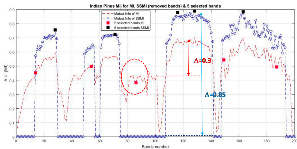
Figure 6. Depicts the I(A, B) of the bands of the Indian Pine dataset given by the MI (red plot) and SSMI (blue plot) BS methods. Note that the SSMI that utilizes both spatial and spectral information enhances the contrast of the I(A, B) by as much as approximately 200% in comparison to the basic MI BS without spatial preprocessing.
