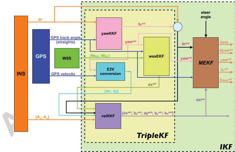
Figure 3: Schematic diagram for the Triple KF and the IKF design
