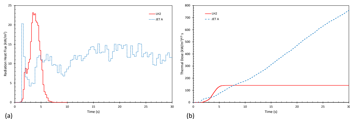
Figure 4 - Comparison of the (a) predicted radiation heat flux and (b) thermal radiation dose produced by the LH2 and Jet A 500 \text{ L} fuel spill pool fires received at a monitor point 15 \text{ m} from the origin of the fire.
