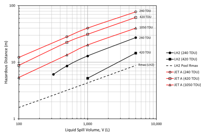
Figure 5 - Comparison of hazardous distance vs. spill volume predicted for LH2 and Jet A fuel spill pool fires, at different thermal dose thresholds.
