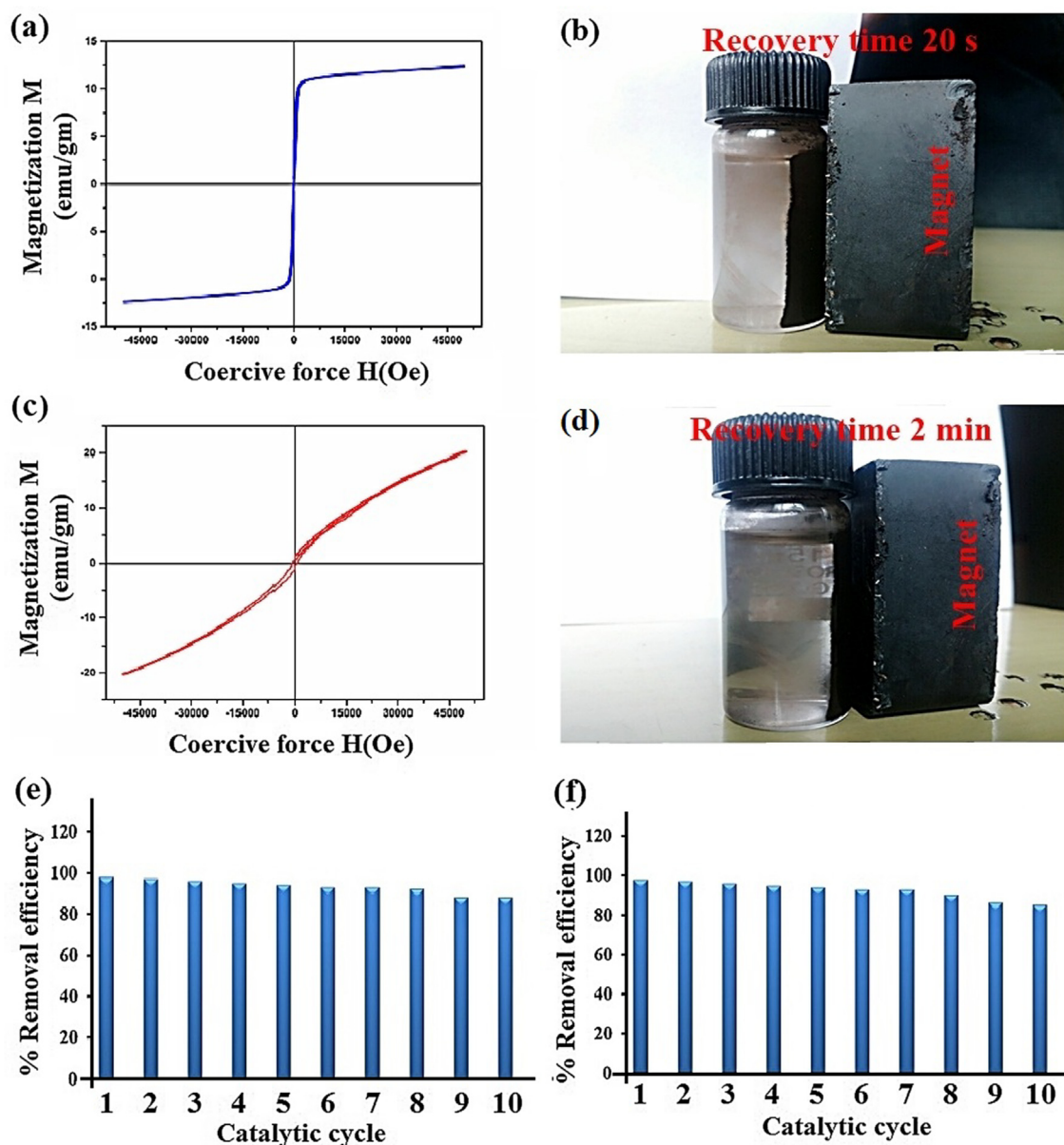
Fig. 9 Hysteresis curve and magnetic separation of ZnO/ZF/NG (a–b), Hysteresis curve and magnetic separation of ZnO/CF/NG (c–d), Recycle efficiency of ZnO/ZF/NG (e) and ZnO/CF/NG (f) for MG removal. Reaction conditions: [MO] = 1.5 \times 10^{-5} \text{ mol dm}^{-3} ; [MG] = 1 \times 10^{-5} \text{ mol dm}^{-3} ; [catalyst] = 50 \text{ mg/100 mL} ; \text{pH} = 4.0(\text{MO}) ; 6 (MG); reaction time = 70 min (MG) and 140 min (MO), Light Intensity = 750 lx.
