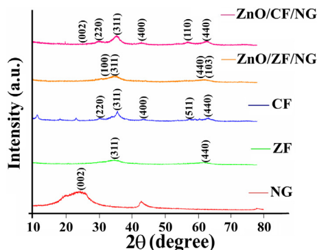
Fig. 1 XRD patterns of NG, ZF, CF, ZnO/ZF/NG and ZnO/CF/NG nanocomposites.
