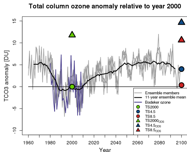
Figure 1. Total-column ozone anomalies (in DU) relative to the year 2000 \pm 5 mean, averaged over 10^{\circ}\text{S} – 10^{\circ}\text{N} for the four transient UM-UKCA experiments following the RCP6.0 future emissions scenario (grey lines), and the ensemble mean 11-year running mean (black line). Coloured circles and triangles represent tropical total-column ozone in the time-slice experiments, as given in the figure legend. The purple line shows tropical averaged total-column ozone values from v2.8 of the Bodeker dataset (Bodeker et al., 2005).
