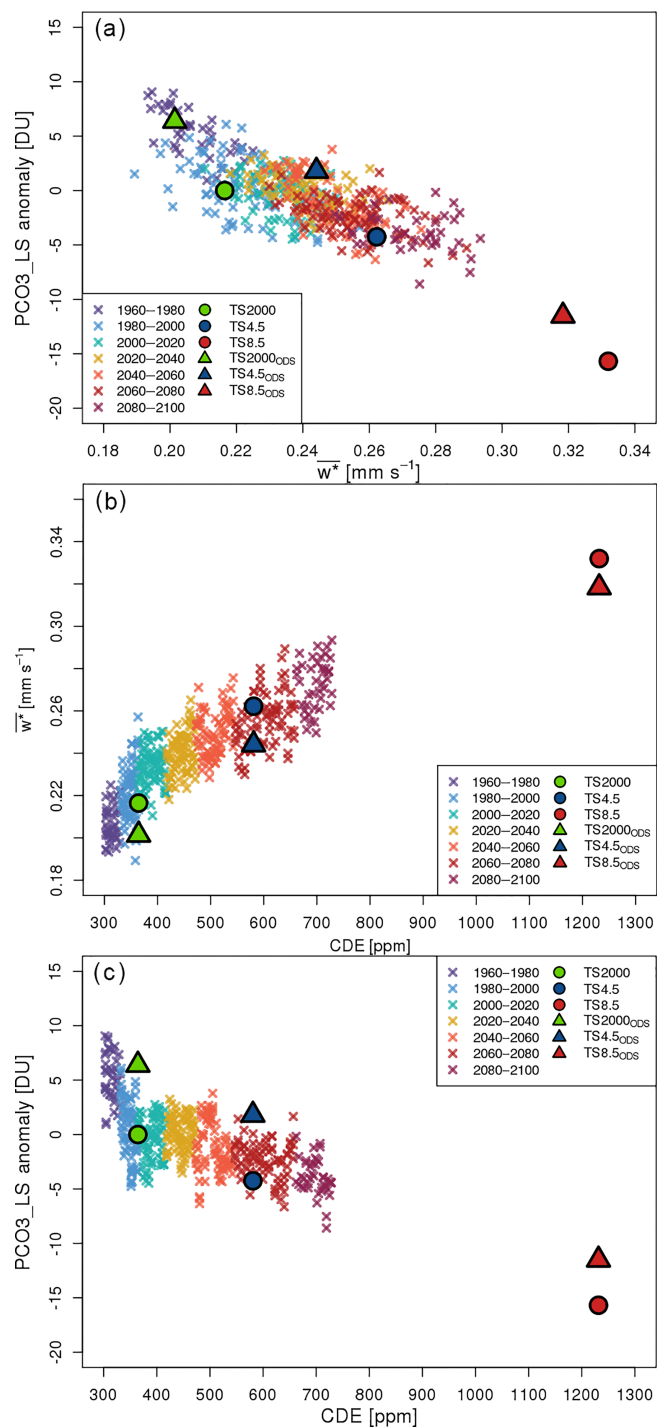
Figure 5. Scatter plot of (a) lower-stratospheric partial-column ozone anomalies relative to the year 2000 \pm 5 mean (in DU) vs. 70 hPa \bar{w}^* (in \text{mm s}^{-1} ), (b) 70 hPa \bar{w}^* vs. CDE mixing ratio (in ppmv) and (c) lower-stratospheric partial-column ozone anomalies vs. CDE mixing ratio for the transient simulations (crosses) and time-slice experiments (circles and triangles). Results from the transient simulations have been coloured in 20-year sections.
