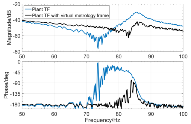
Figure 3. Comparison of the plant Transfer Function (TF) measurements with and without the virtual metrology frame.
