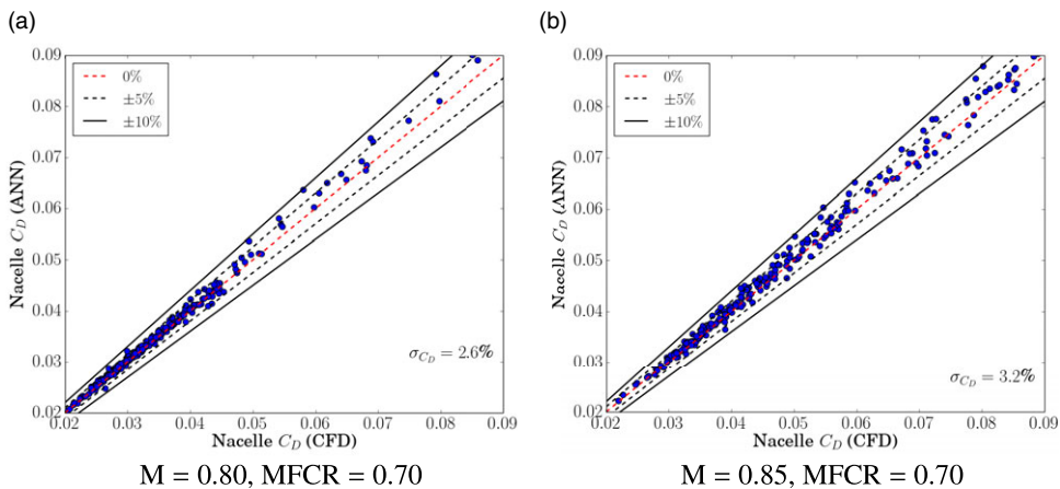
Figure 6. ANN cross validation for medium- and long-range applications at mid-cruise conditions.
