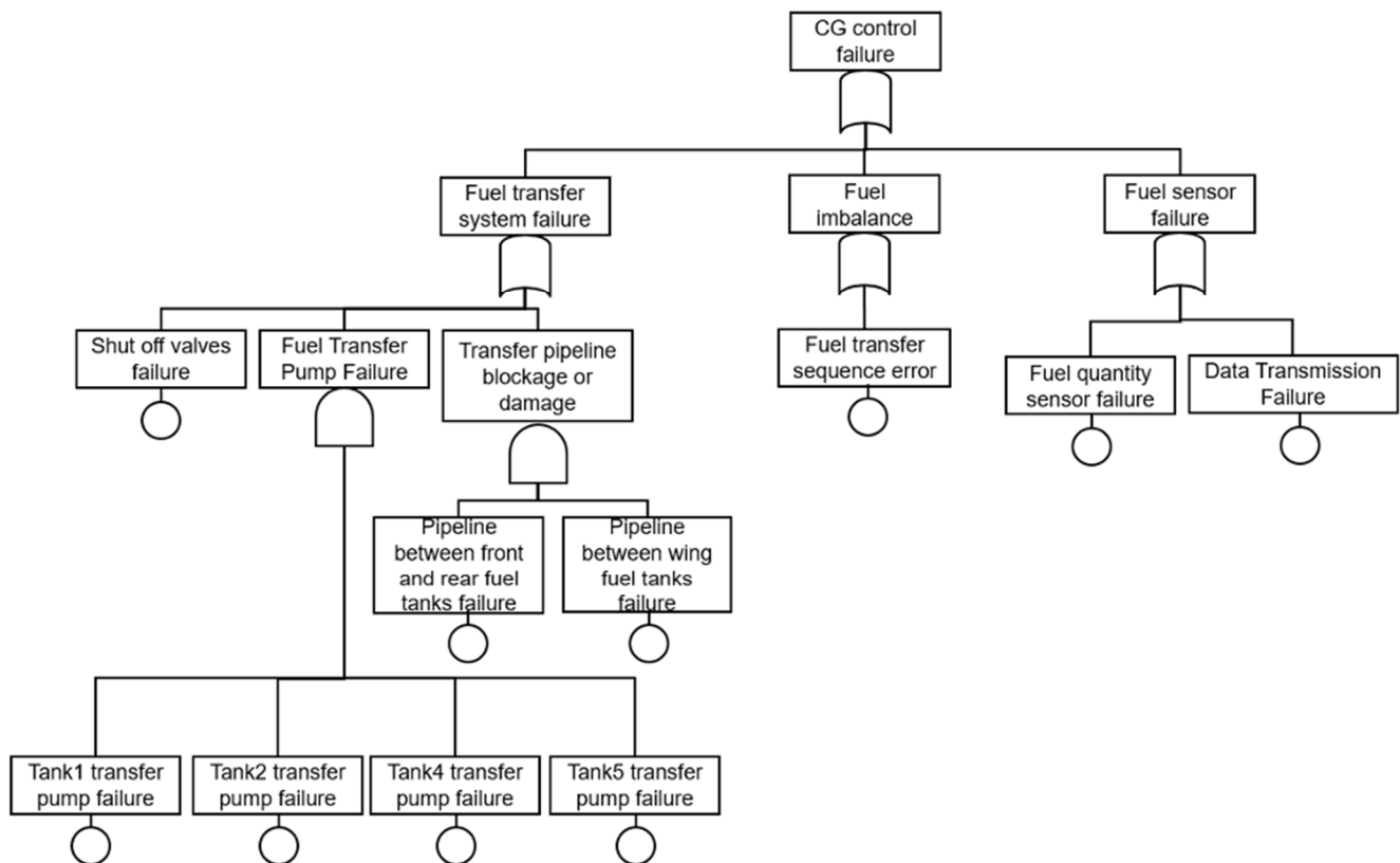
Figure A5. Fault tree diagram illustrating the causes leading to centre of gravity (CG) control failure in the aircraft fuel system. Rectangular blocks represent system and intermediate events, circular nodes denote basic failure events, AND gates indicate that all input events must occur simultaneously to trigger the output event, while OR gates indicate that any single input event can lead to the output condition.
