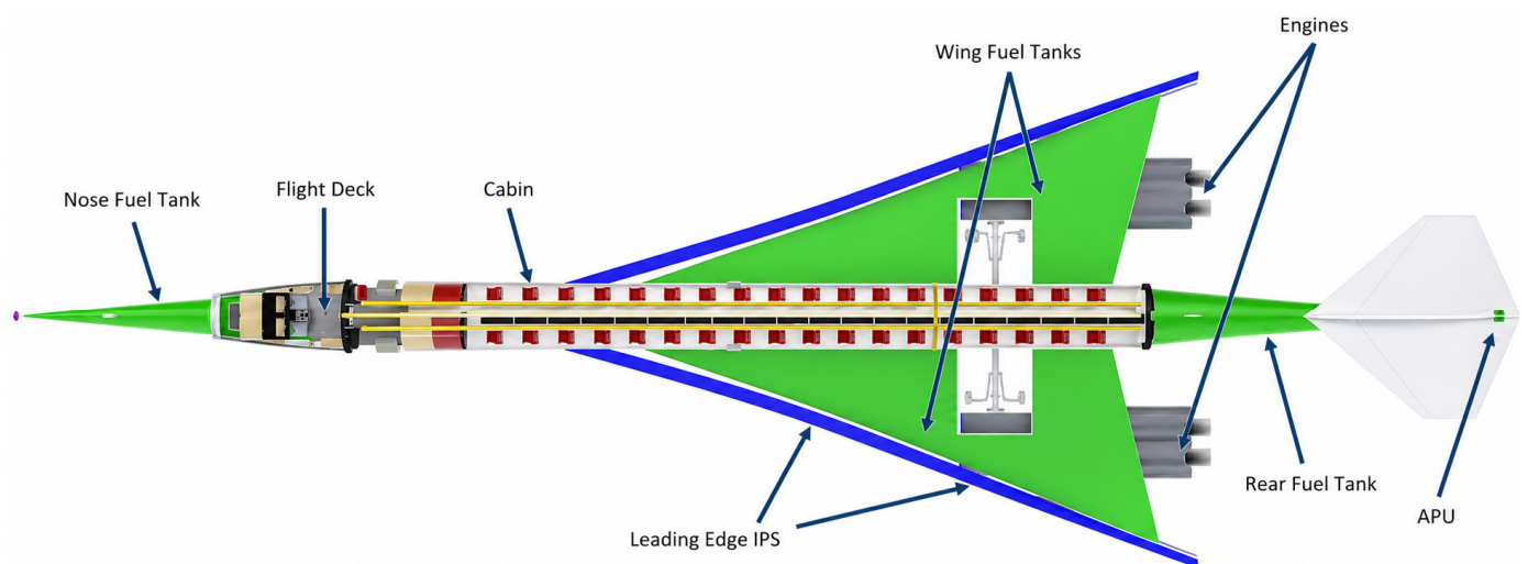
Figure 8. Annotated system-level layout of the SA-24 Phoenix aircraft highlighting fuel system components, subsystem distribution, and key interaction zones relevant to zonal hazard analysis.
