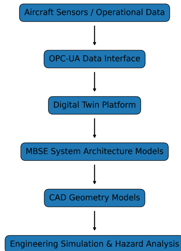
Figure 10. Digital thread architecture for integrated CAD–MBSE systems.
