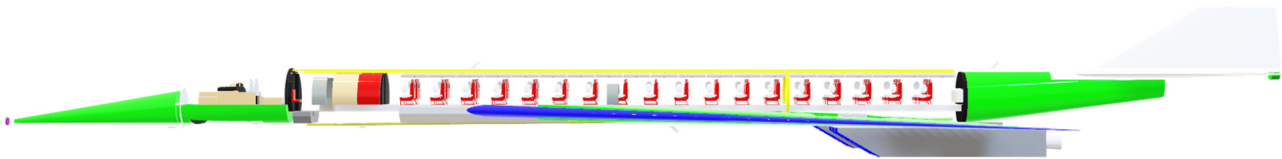
Figure 9. Side view of the system-level layout of the SA-24 Phoenix aircraft.
