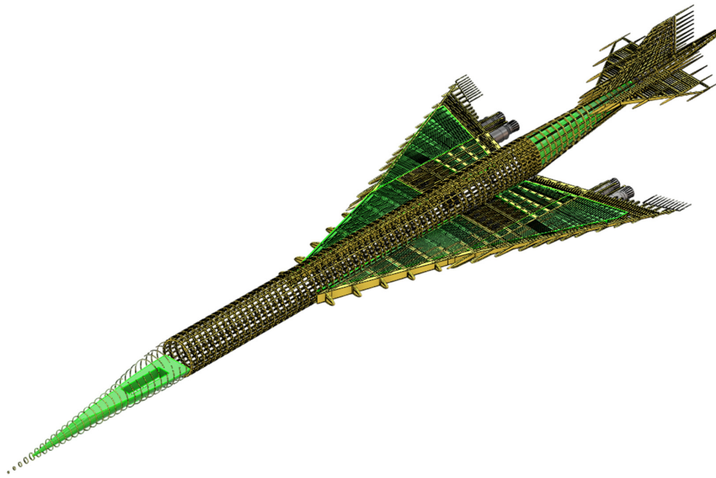
Figure 7. Perspective view of the structure and fuel tank system of the SA-24 aircraft.
