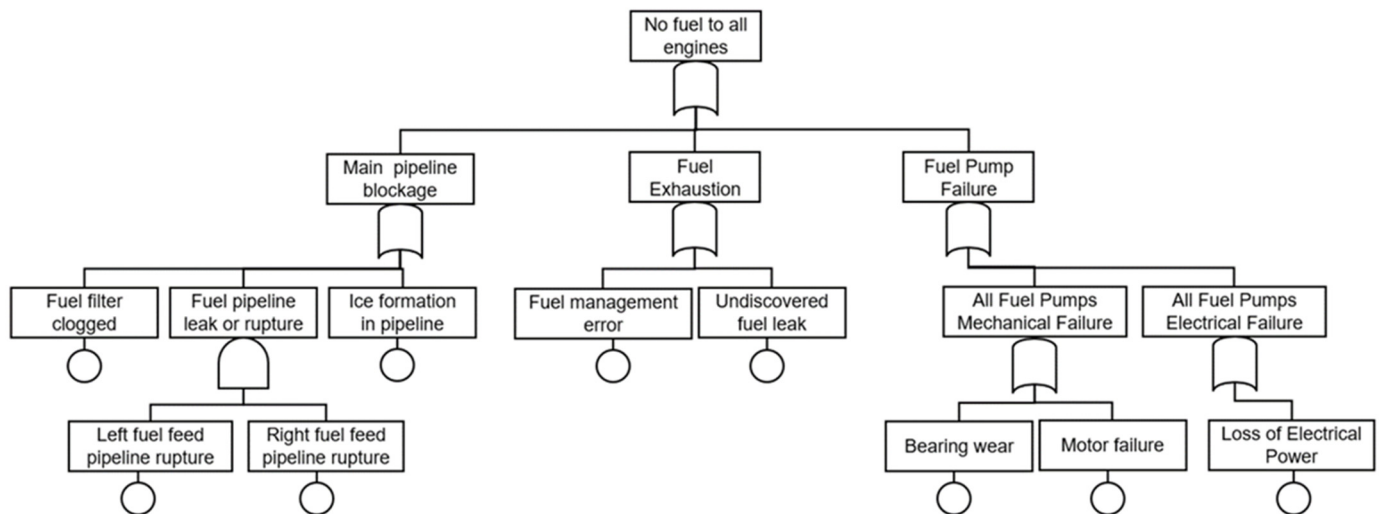
Figure A4. Fault tree diagram illustrating the causes leading to the “no fuel to all engines” failure condition. Rectangular blocks represent system events, circular nodes denote basic failure events, AND gates indicate that all input events must occur simultaneously to trigger the output event, while OR gates indicate that any single input event can lead to the output condition.
