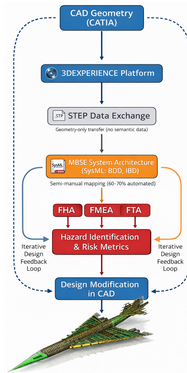
Figure 1. CAD–MBSE integration workflow.
