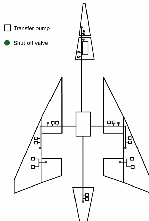
Figure 6. Fuel transfer and shut-off valve system layout of SA-24 Phoenix.
