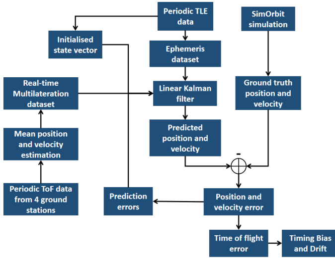
Fig. 1. Solution methodology overview
