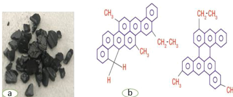
Fig. 2 – Pitch: (a) physical appearance, and (b) chemical components found in pitch-derived from crude oil/petroleum.
