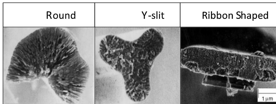
Fig. 15 – Scanning electron microscope photographs of carbonised fibres spun through different shaped nozzles [84].
