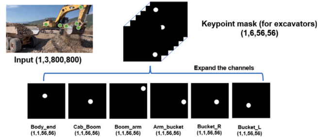
Fig. 5. An example for encoding the keypoints in the output mask on an excavator. There are 6 ( K=6 ) one-hot 56 \times 56 binary masks, each of which has only a single pixel labelled as the object.
