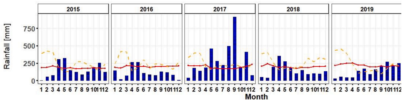
Fig. B2. Monthly rainfall (blue bars), mean temperature (red line) and mean solar radiation (orange dashed line) at Kericho tea estate (Kenya). (For interpretation of the references to colour in this figure legend, the reader is referred to the web version of this article.)
