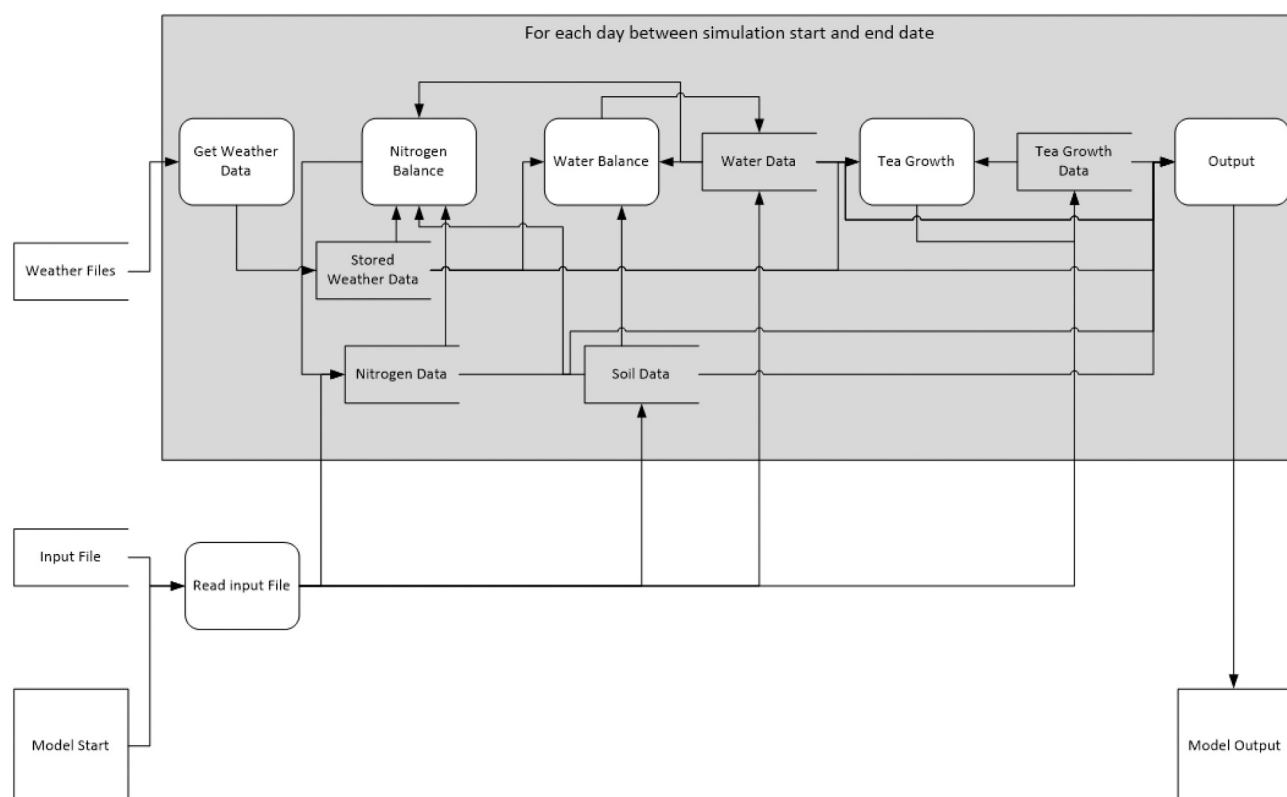
Fig. A1. Top-level diagram showing overview of CUPPA-Tea model.
