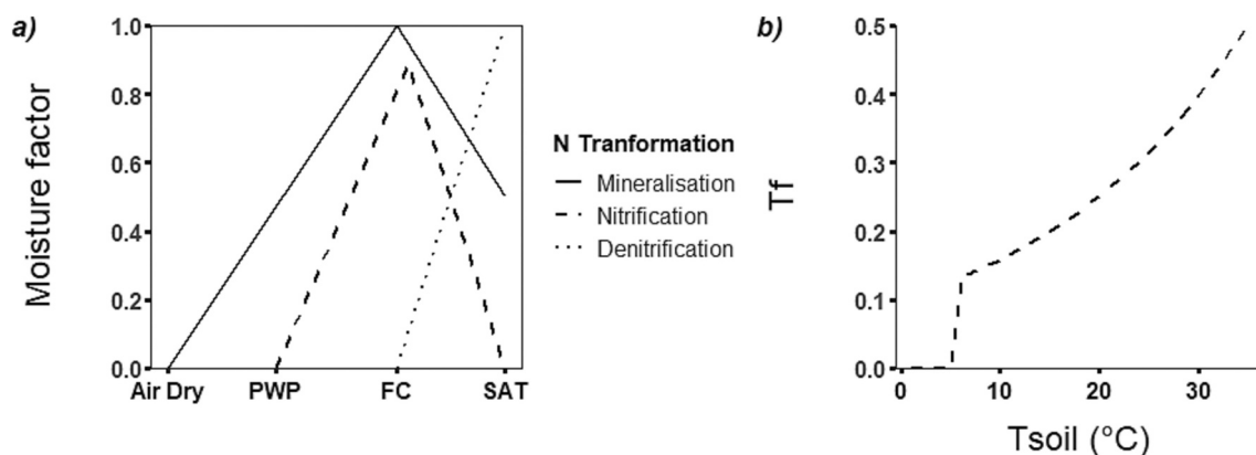
Fig. 4. a) Soil water indices used in CUPPA-Tea to modify soil N transformation rates (PWP: permanent wilting point, FC: field capacity, SAT: saturation moisture content, (adapted from Godwin and Jones, 1991) and b) soil temperature factor response used in CUPPA-Tea denitrification routine.
