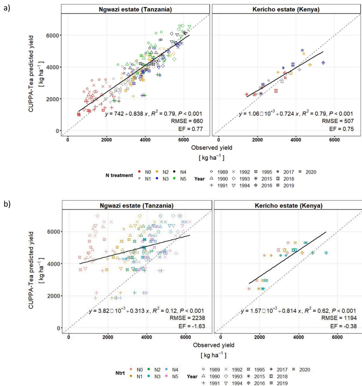
Fig. A3. Comparison of CUPPA-Tea goodness of fit for Ngwazi and Kericho when the N routine is a) turned on and b) turned off (Dashed line: 1:1; RMSE: root mean square error; EF: Modelling efficiency; shapes indicate year and colors N treatment).
