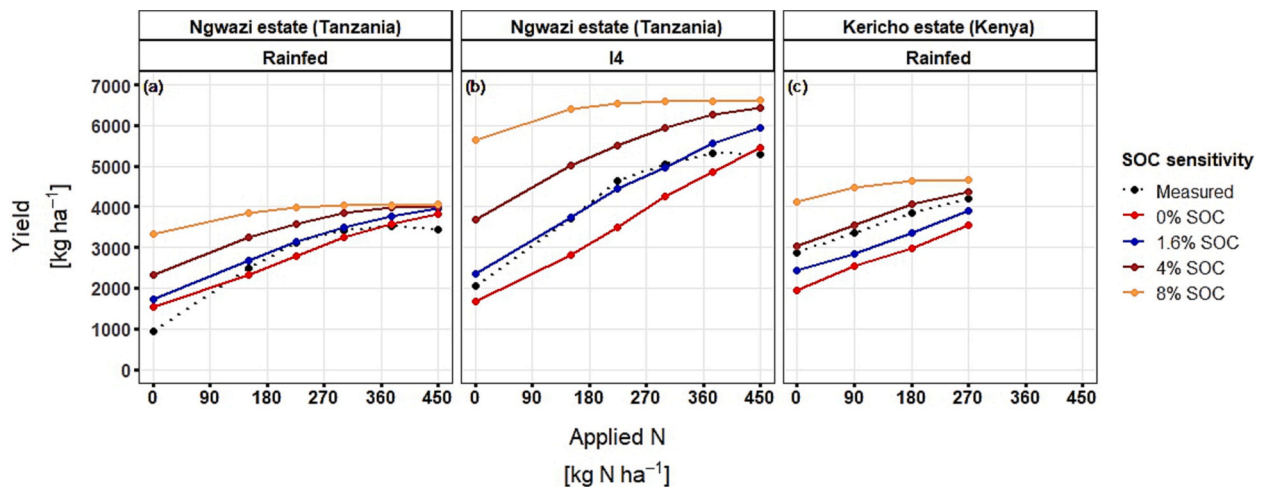
Fig. 7. Predicted effect of soil organic carbon (SOC) content (0, 1.6, 4 and 8%) on the tea yield response to nitrogen application in unpruned years (mean yields of unpruned years) for a) rainfed tea and b) fully irrigated tea in Tanzania (I4), and c) rainfed tea in Kenya. Default SOC values for Ngwazi and Kericho were 1.6% and 4% respectively.
