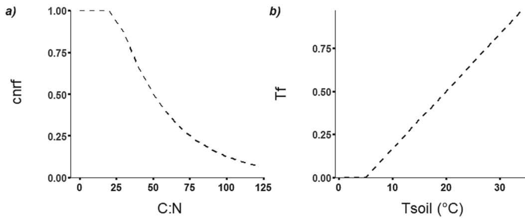
Fig. 2. Response of a) the C:N ratio factor ( cnrf ) to the soil C: N ratio, and b) the soil temperature factor ( Tf ) to soil temperature ( T_{soil} ) assumed in the CUPPA-Tea mineralization routine.
