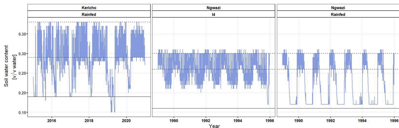
Fig. A2. Daily simulated soil water content at Kericho (under rainfed conditions at the top 15 cm) and at Ngwazi (under rainfed and I4 treatment at the top 25 cm). Solid line shows the permanent wilting point, dashed line the field capacity and dotted line is the saturated water content.
