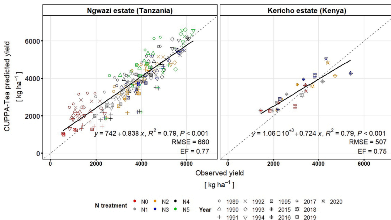
Fig. 6. Linear regression analysis of the predicted yields using the CUPPA-Tea model with observed yields from a) Ngwazi Estate in Tanzania (1989–1995) and b) Kericho Estate in Kenya (2015–2020) experiments (Dashed line: 1:1; RMSE: root mean square error; EF: Modelling efficiency; shapes indicate year and colors N treatment).
