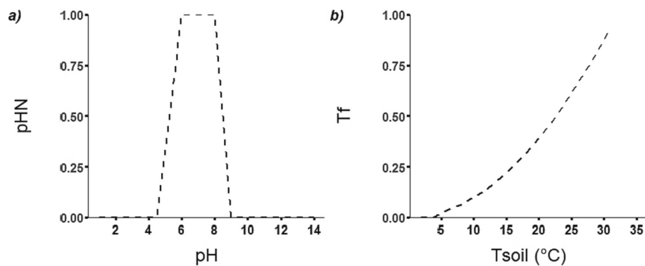
Fig. 3. Response of a) a pH factor ( pHN ) to pH and b) a soil temperature factor ( Tf ) to temperature in the CUPPA-Tea nitrification routine.
