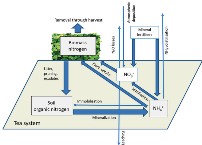
Fig. 1. Schematic diagram showing the main stocks and flows of nitrogen between the soil and the tea crop.
