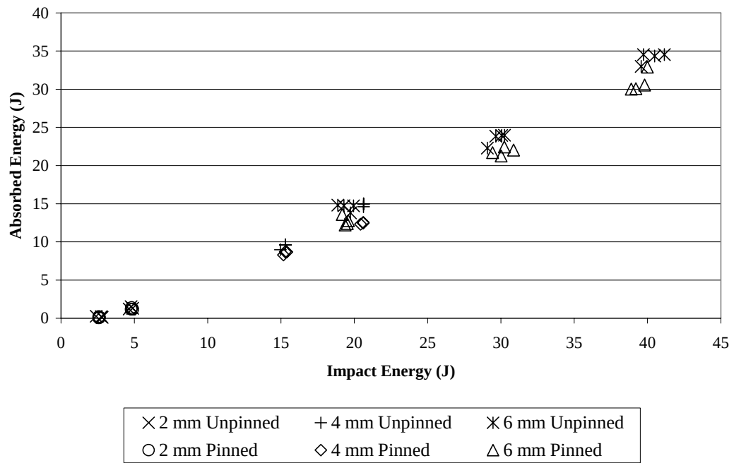
Fig. 7 Absorbed energy versus impact energy.
