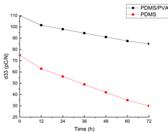
Figure 4. Piezoelectricity d_{33} decay cures for 72 hours
