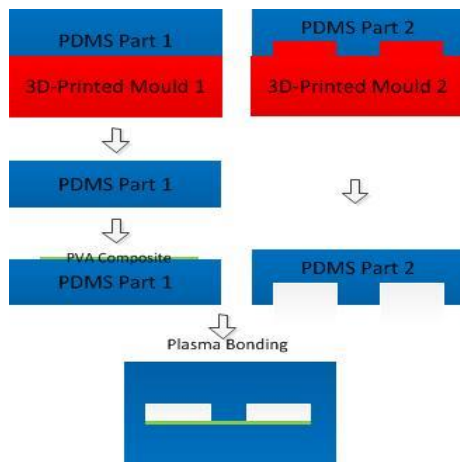
Figure 2. Schematic of fabrication processes
