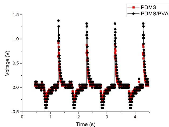
Figure 5. Measured voltage output for PDMS and PDMS/PVA ferroelectret at 1 hour after corona charging
