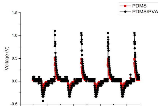
Figure 6. Measured voltage output for PDMS and PDMS/PVA ferroelectret at 72 hour after corona charging
