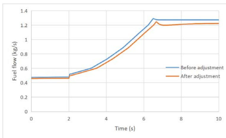
Figure 27. Comparison of the fuel flow to the degraded engine before and after adjustment of the controller.
