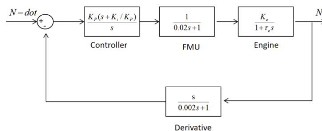
Figure 15. Block diagram for N-Dot loop.
