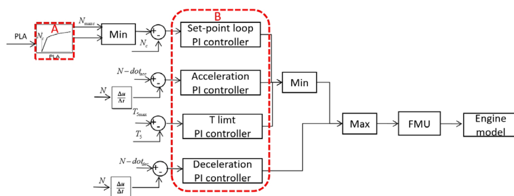
Figure 14. Architecture of a Min-Max controller.
