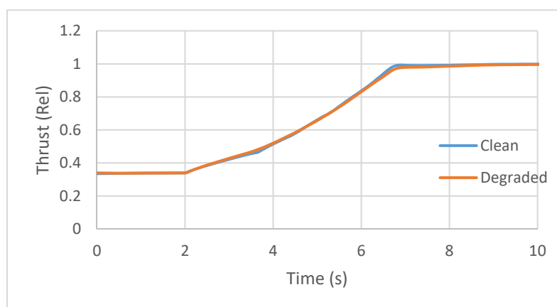
Figure 25. Comparison of the thrust of the clean engine with the clean controller and the degraded engine with the adjusted controller.
