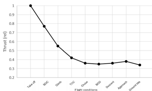
Figure 17. Thrust requirement for different flight conditions. BOC: beginning of climb; TOC: top of climb; and BOD: beginning of descent.
