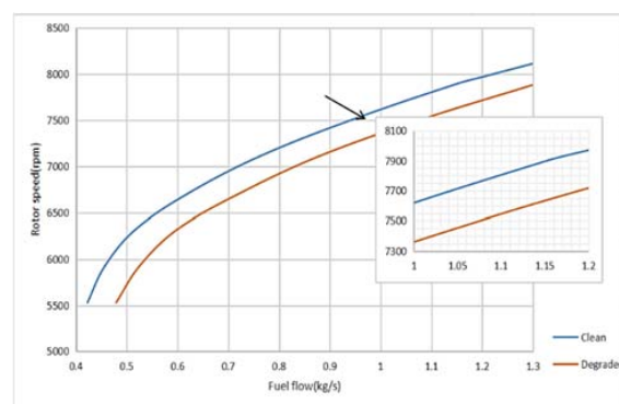
Figure 20. Comparison of the fuel flow to rotor speed relationship between a clean engine and degraded engine.
