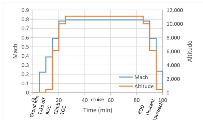
Figure 16. Flight conditions in a typical flight mission.
