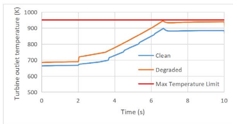
Figure 26. Comparison of the turbine outlet temperature of the clean engine with the clean controller and the degraded engine with the adjusted controller.
