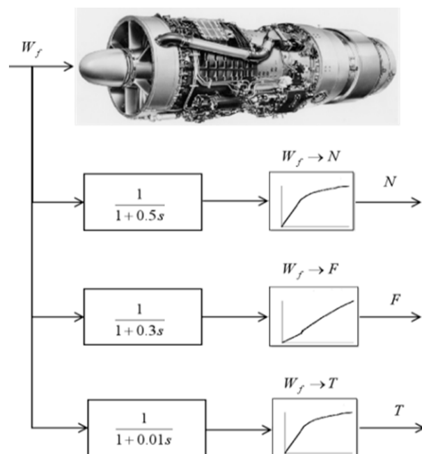
Figure 13. Wiener model for an AVON engine.
