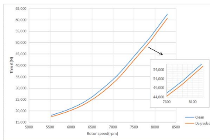
Figure 19. Comparison of the rotor speed to thrust relationship between a clean engine and degraded engine.
