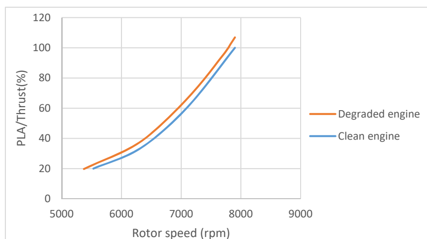
Figure 23. Adjustment of the PLA to rotor speed relationship of the degraded engine.
