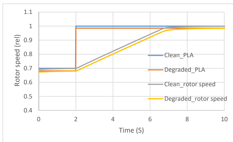
Figure 24. Comparison of the rotor speed of the clean engine with the clean controller and the degraded engine with the adjusted controller.
