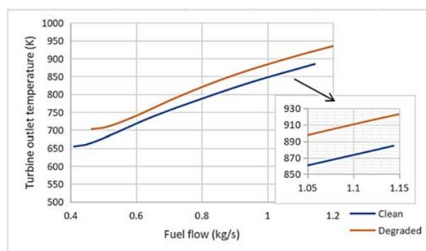
Figure 21. Comparison of the fuel flow to turbine temperature relationship between a clean engine and degraded engine.
