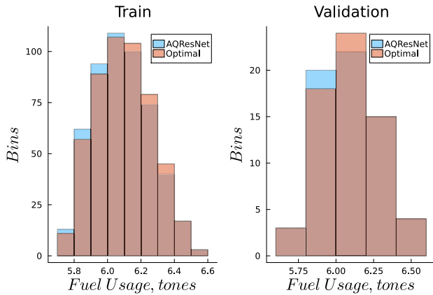
FIGURE 12. Fuel consumption histograms for AQResNet.
