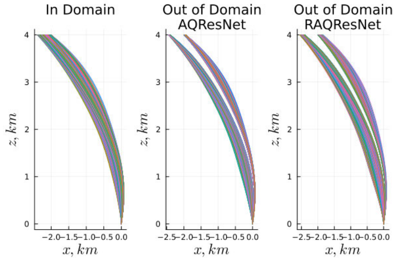
FIGURE 11. Trajectories driven by (R)AQResNet neural network models.
