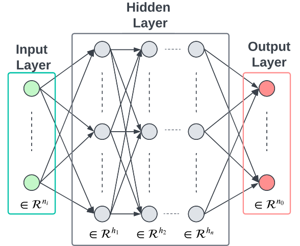
FIGURE 5. General deep neural network architecture.
