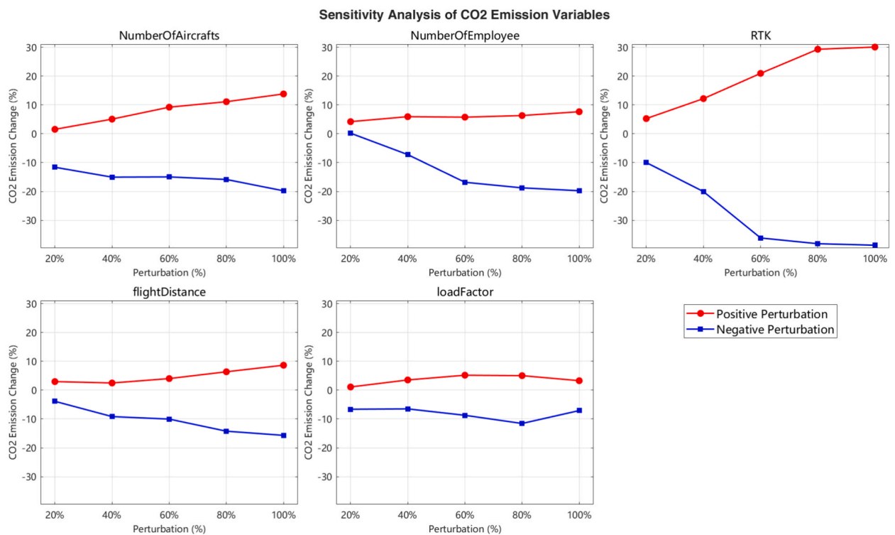
Fig. 5.13. Sensitivity analysis of CO 2 emission variables.
