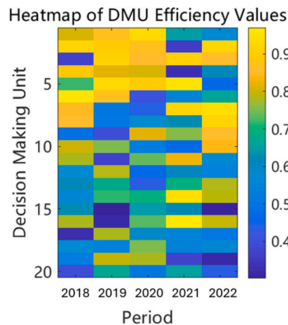
Fig. 6.5. Heatmap of DMU Efficiency Values (2018–2022).
