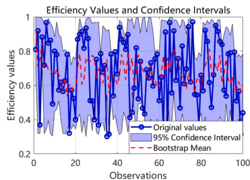
Fig. 6.4. GML Bootstrap efficiency values and confidence intervals.
