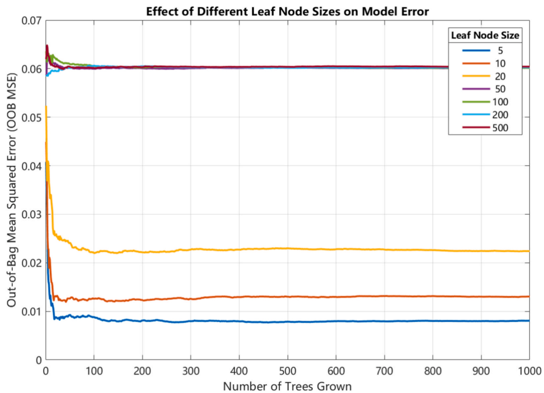
Fig. 5.9. Out-of-bag error curves for different minimum leaf sizes.
