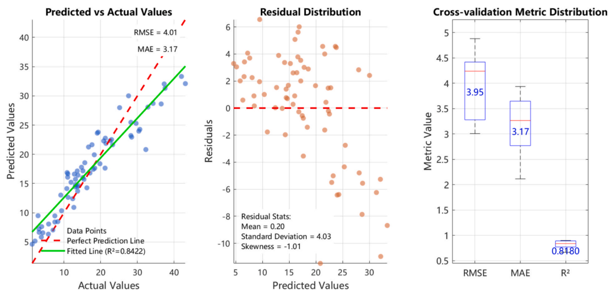
Fig. 5.10. Cross-validation results for the Random Forest model.
