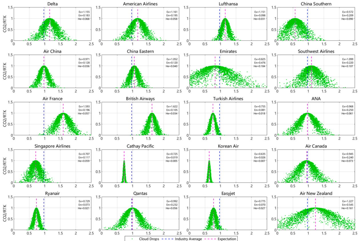
Fig. 5.1. Carbon Intensity Index of CO 2 /RTK for 20 global airlines.
