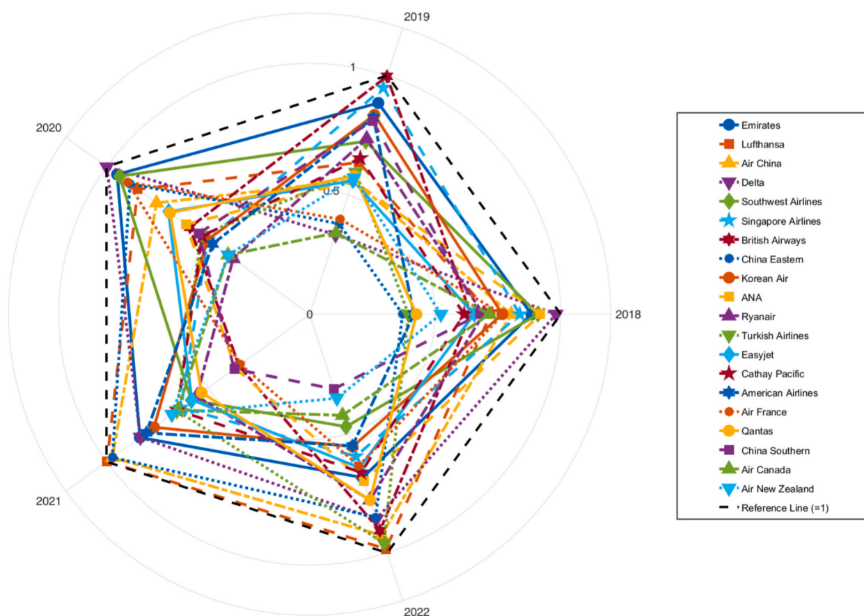
Fig. 6.1. Efficiency scores of the 20 airlines from the SBM-DDF model (2018–2022).
