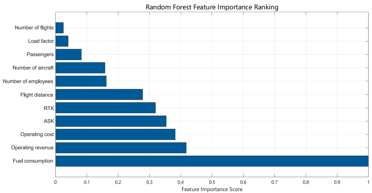
Fig. 5.7. Random Forest importance ranking.
