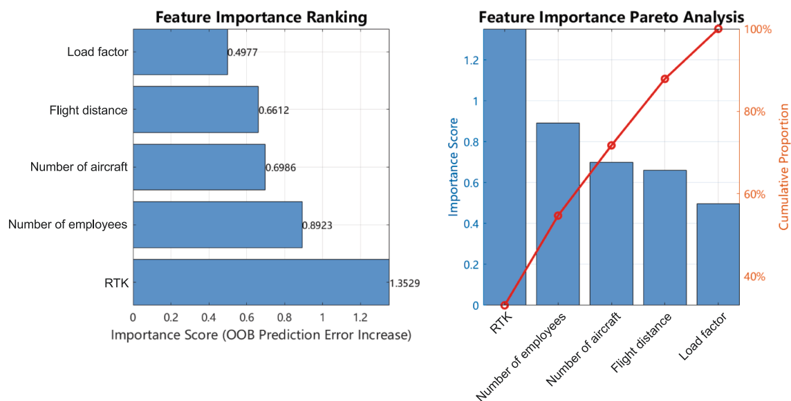
Fig. 5.11. Mean Decrease Impurity (MDI) variable importance rankings.
