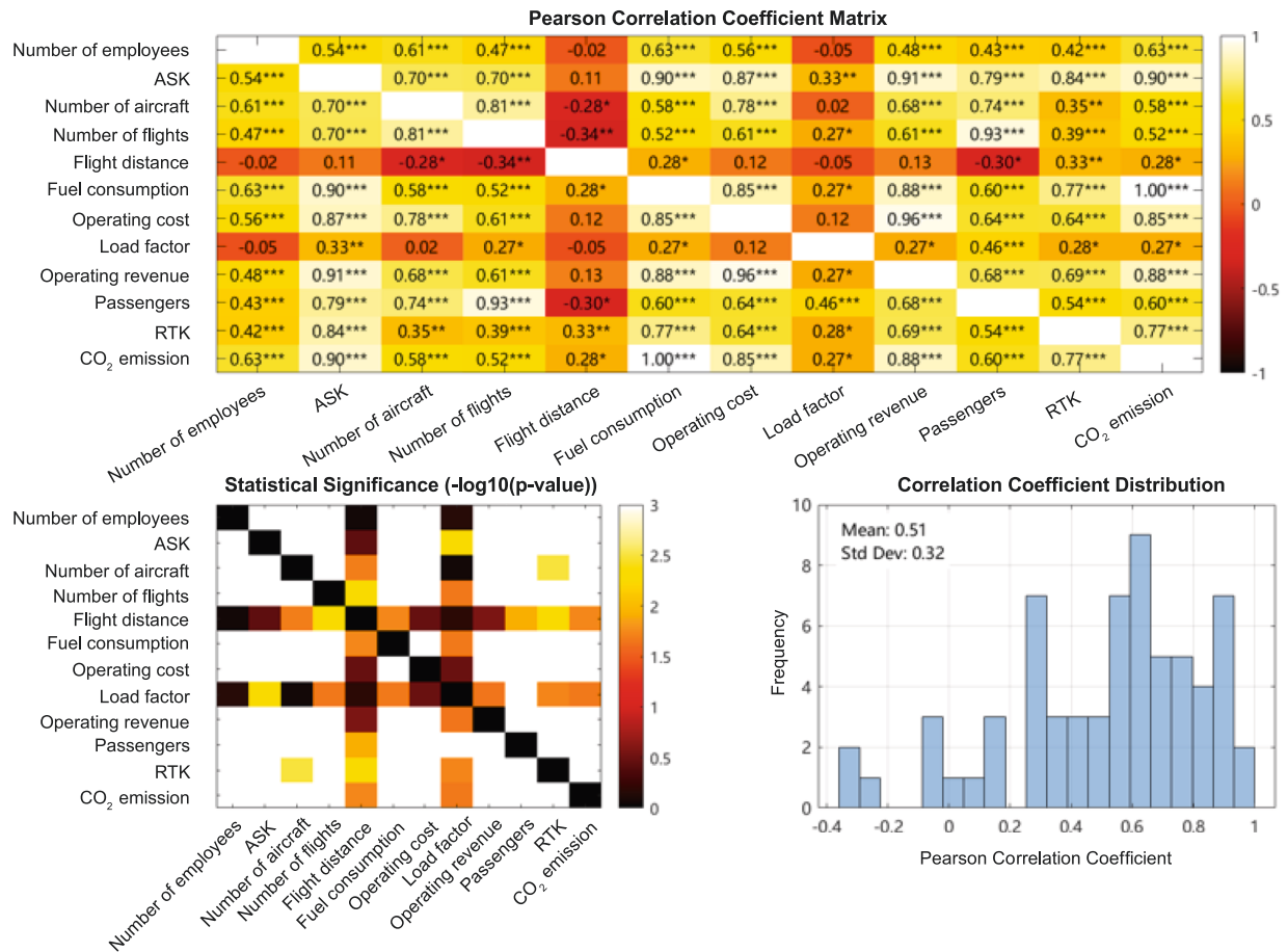
Fig. 5.5. Pearson correlation matrix of candidate indicators.
