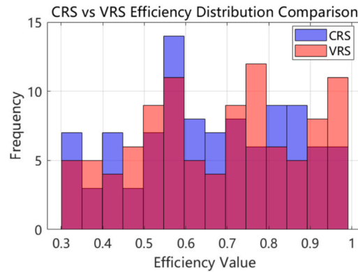
Fig. 7.2. Comparison of CRS and VRS efficiency results under the SBM-DDF model.
