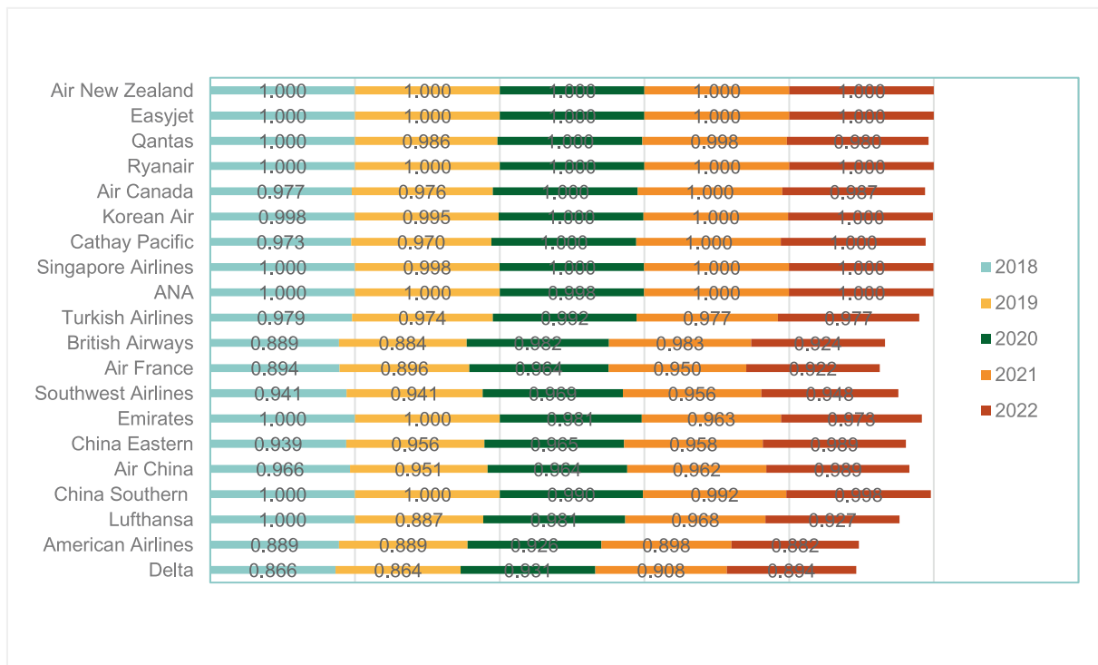
Fig. 6.3. EEI scores for the 20 global airlines during 2018–2022.
