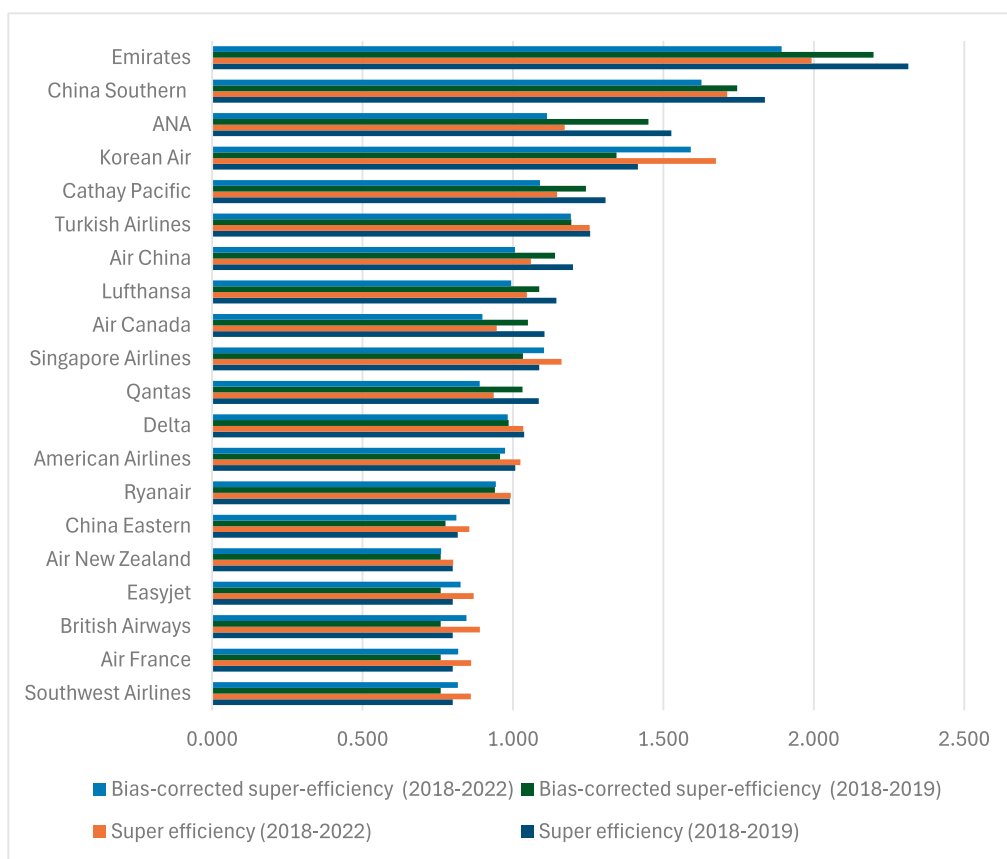
Fig. 7.1. Comparison of average super-efficiency and bias-corrected super-efficiency scores under pre-COVID (2018–2019) and full-sample (2018–2022) datasets.
