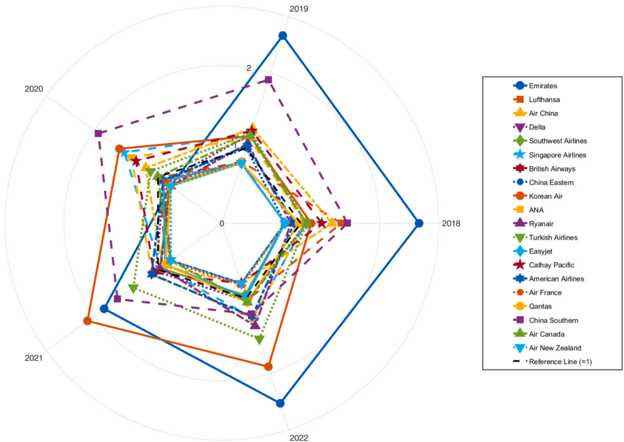
Fig. 6.2. Efficiency scores of the 20 airlines from the Super-SBM model (2018–2022).
