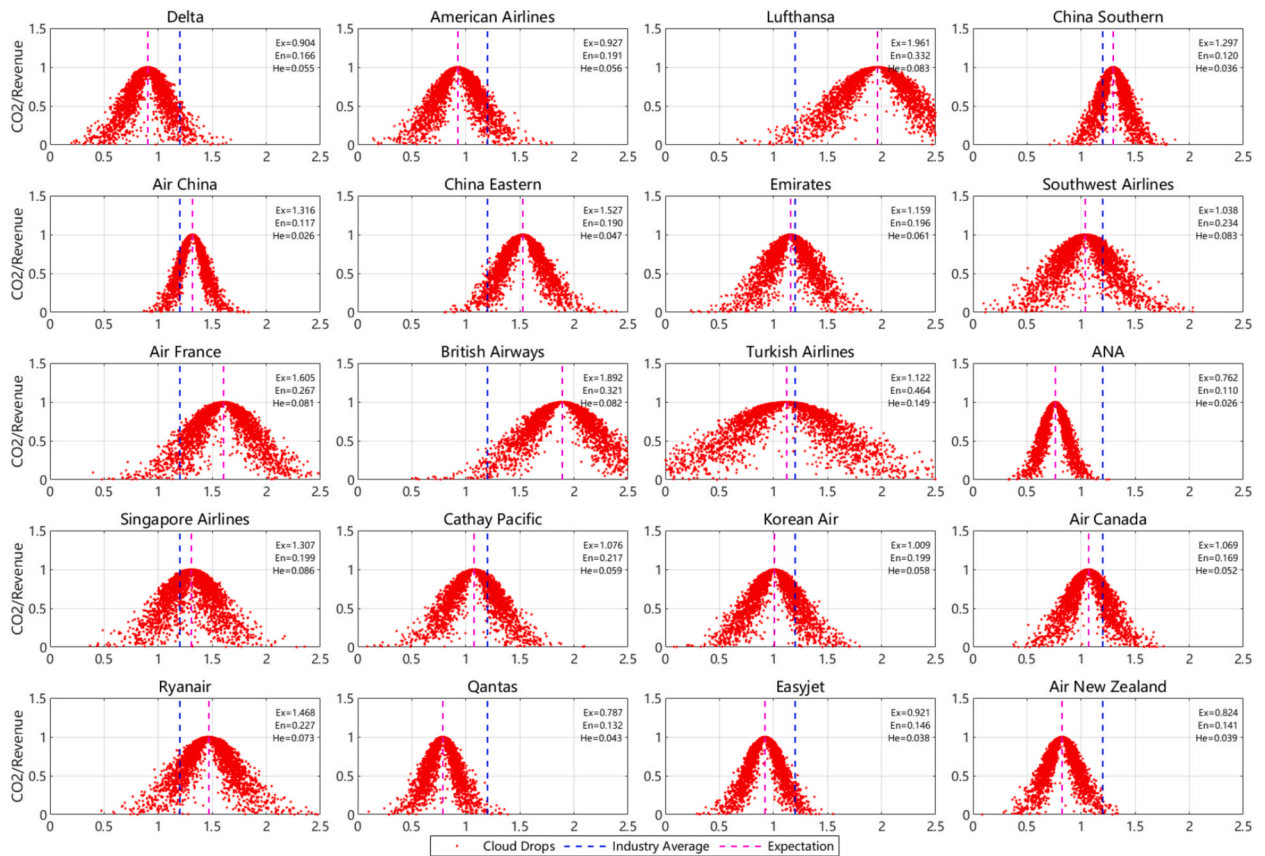
Fig. 5.3. Carbon Intensity Index of CO2 per unit of operating revenue for 20 global airlines.
