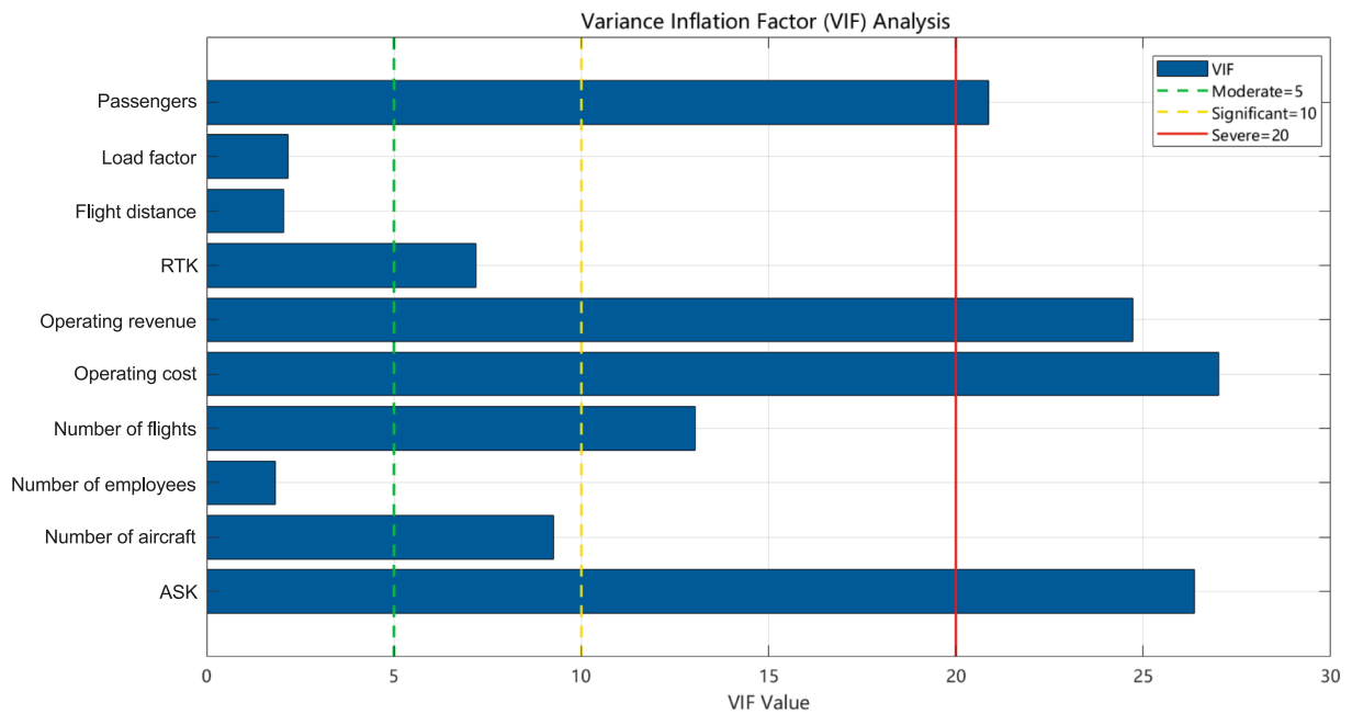
Fig. 5.8. Variance Inflation Factor (VIF) analysis for dimensionality reduction.
