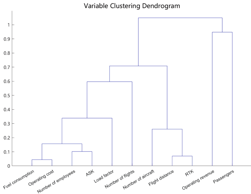
Fig. 5.6. Variable Clustering Dendrogram.
