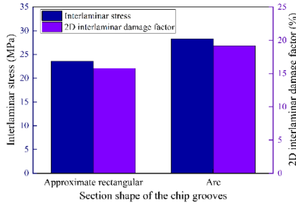
Fig. 14. Interlaminar stress and 2D interlaminar damage factor with different section shape of the chip grooves (fiber orientation angle= 45^\circ , n=4000\text{rpm} , f=0.24\text{ mm}\cdot\text{r}^{-1} , a_p=2\text{mm} , a_e=1\text{mm} )
