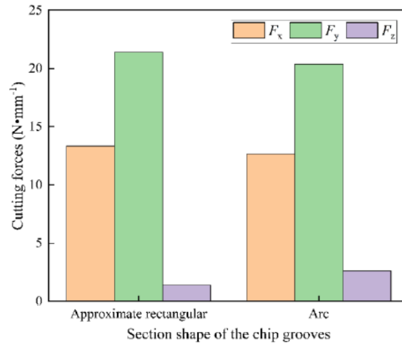
Fig. 13. Cutting forces with different section shape of the chip grooves (fiber orientation angle= 45^\circ , n=4000\text{rpm} , f=0.24\text{ mm}\cdot\text{r}^{-1} , a_p=2\text{mm} , a_e=1\text{mm} )
