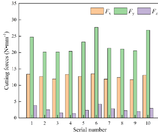
Fig. 9. Cutting forces with different left helix angles and number of the left-handed chip grooves (fiber orientation angle= 45^\circ , n=4000\text{rpm} , f=0.24\text{ mm}\cdot\text{r}^{-1} , a_p=2\text{mm} , a_e=1\text{mm} )
