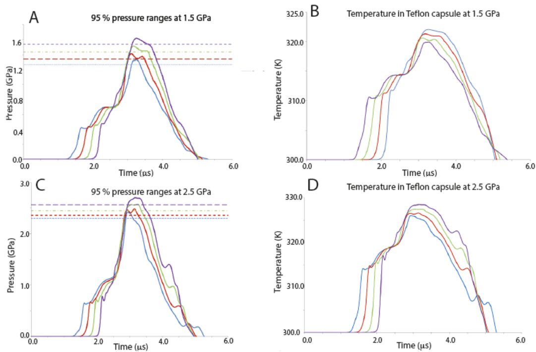
203 Figure 2. Results of modelling experiments carried out to determine pressure and 204 temperature conditions developed as a function of time during shock compression at 205 273 and 360 m/s using ANSYS® Autodyn® simulations. A. Calculated pressures 206 developed within the sample as a function of time for a peak impact pressure of 1.5 207 GPa; B. Calculated temperatures developed within the sample at an impact pressure 208 of 1.5 GPa; C. Calculated pressure-time trace for a shock with peak impact pressure 209 of 2.5 GPa; D. Calculated T profile for an impact pressure of 2.5 GPa. Different 210 coloured lines refer to different P,T profiles at different gauge points within the 211 simulations, selected to estimate the range of P,T conditions developed at various 212 points throughout the sample volume, and thus provide an estimate of the range of 213 values that are expected to exist at various stages during the shock compression event. 214
