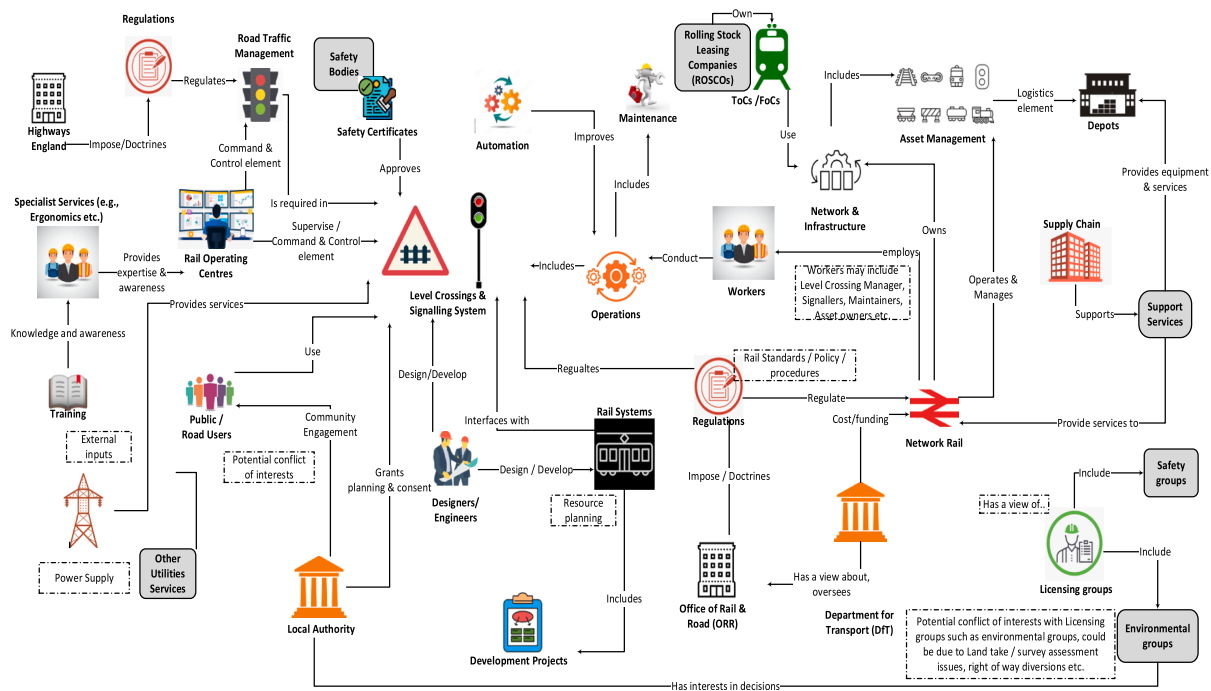
Fig. 3. Rich picture.
