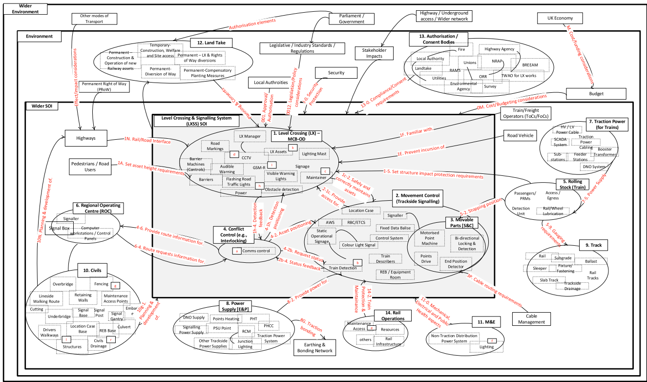
Fig. 4. Context diagram.
