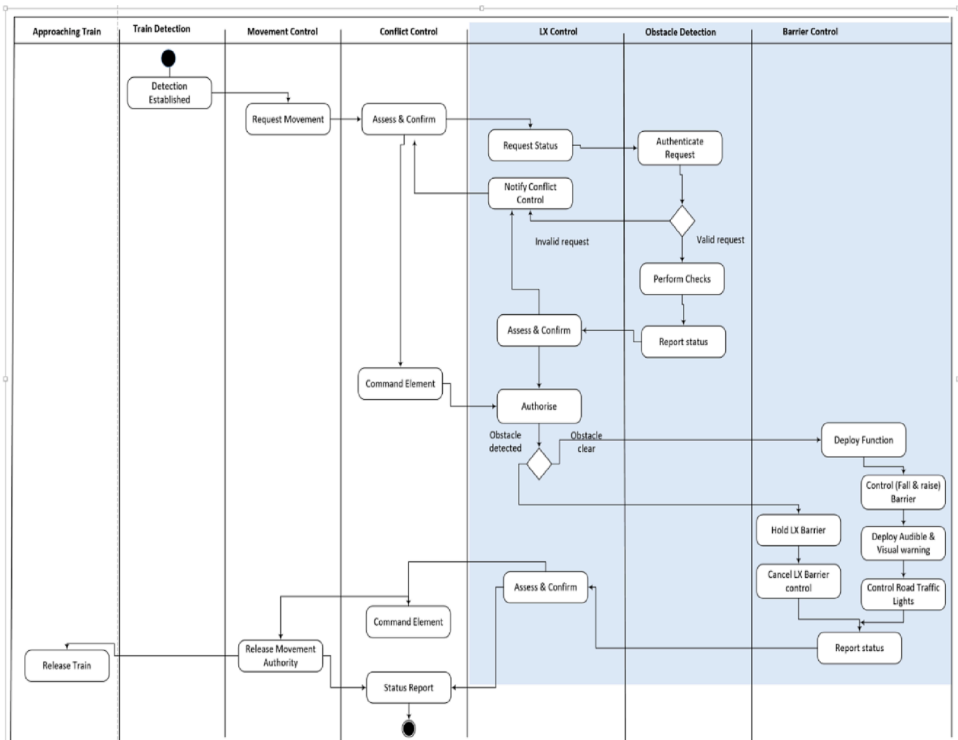
Fig. 8. Activity diagram.
