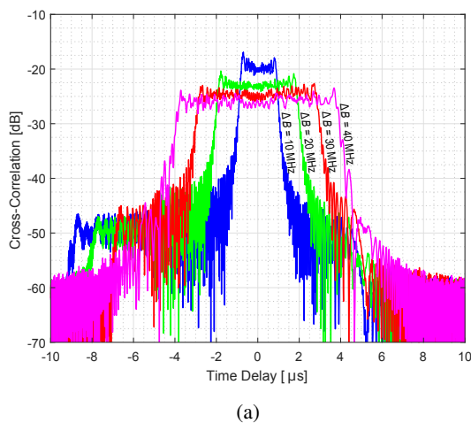
Fig. 8: Experimental results for rectangular LFM signals a Amplitude of the cross-correlation between up-chirps with different bandwidths b Response of the matched filter in the presence of an orthogonal interfering LFM signal
