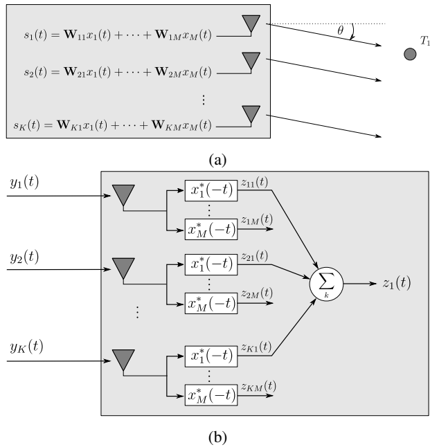
Fig. 1: Schematics of a multibeam radar
