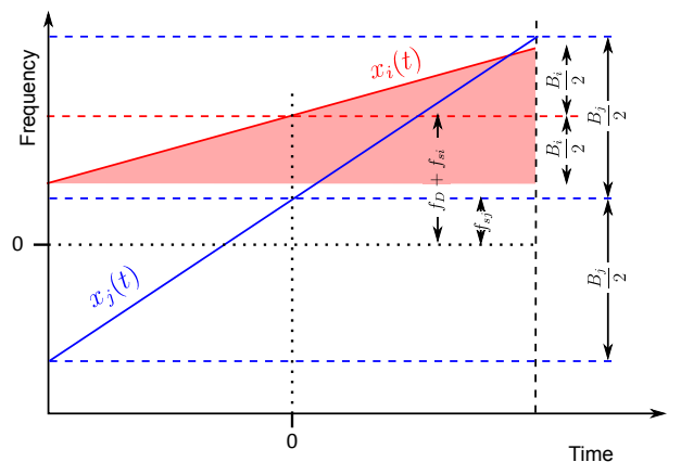
Fig. 2: Time-frequency diagram of two LFM signals
