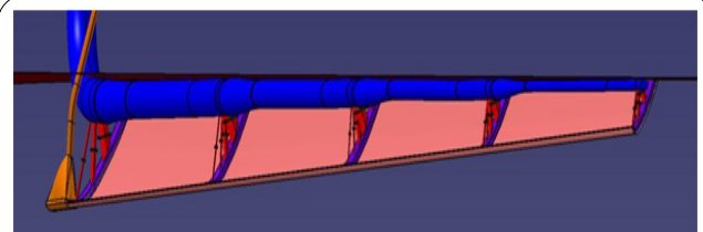
Figure 9: Duct located close to front spar.
