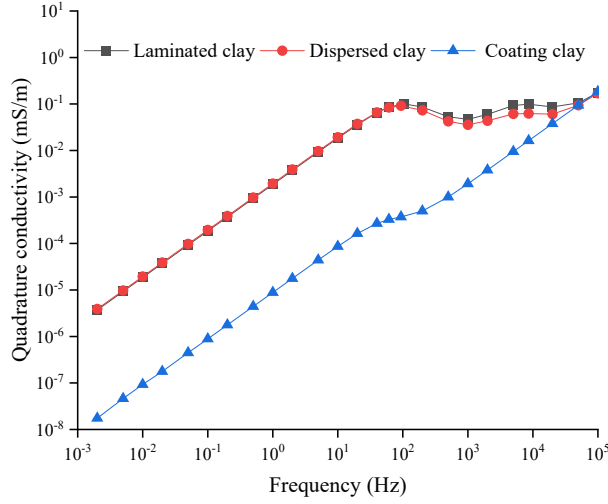
(b) Quadrature conductivity
