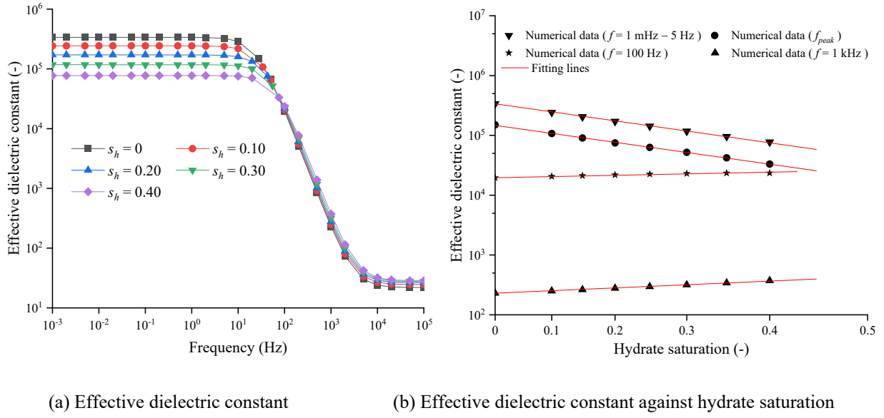
Fig. 11 Effective-dielectric-constant spectra of hydrate-bearing kaolinite with various hydrate saturations
