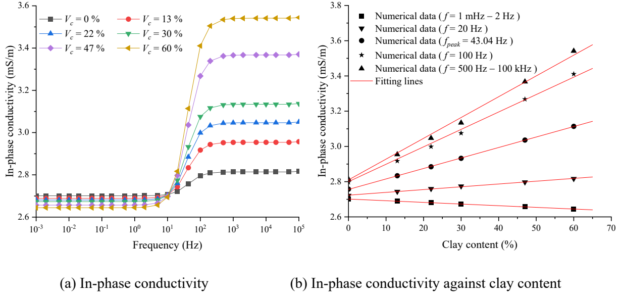
Fig. 7 In-phase conductivity spectra of hydrate-bearing kaolinite and relation with the clay content
