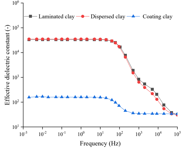
(c) Effective dielectric constant
