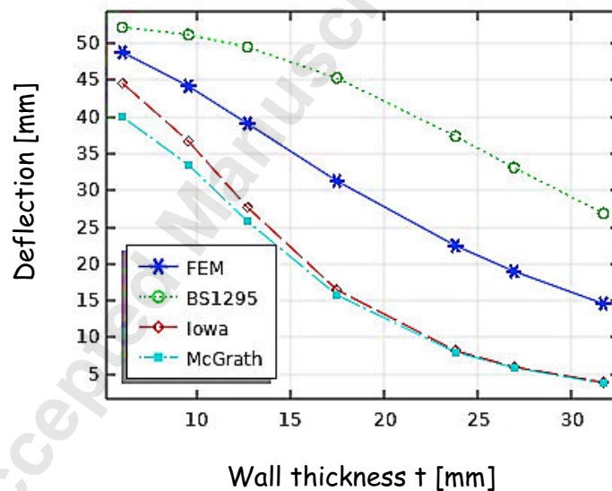
Figure 7. Deflection results of intact buried pipe for proposed model (FEM) and available design standards
