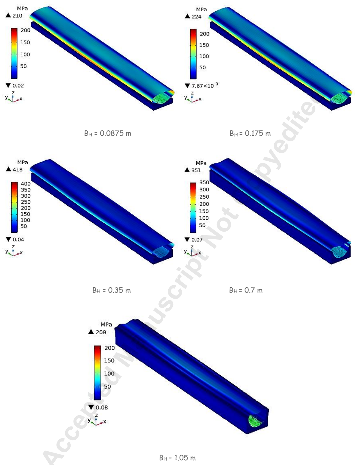
Figure 14. von Mises stresses of corroded pipeline ( t = 6 \text{ mm} ; t_1 = 0.8t ; Q = 60^\circ ) for different bedding depths ( B_H )
