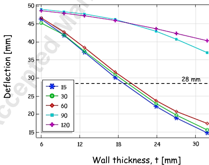
Figure 8. Deflection for buried pipeline with defect damage at pipes invert for different spread angles
