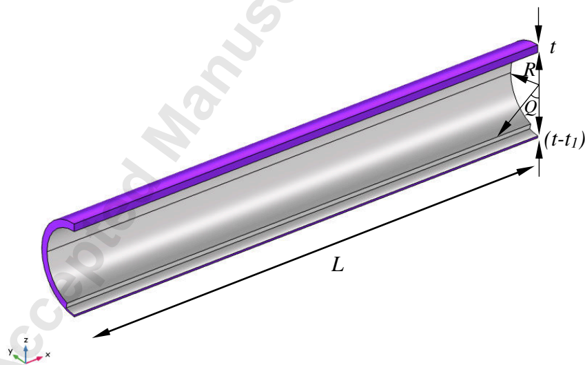
Figure 4. Pipeline and defect geometric parameters.
