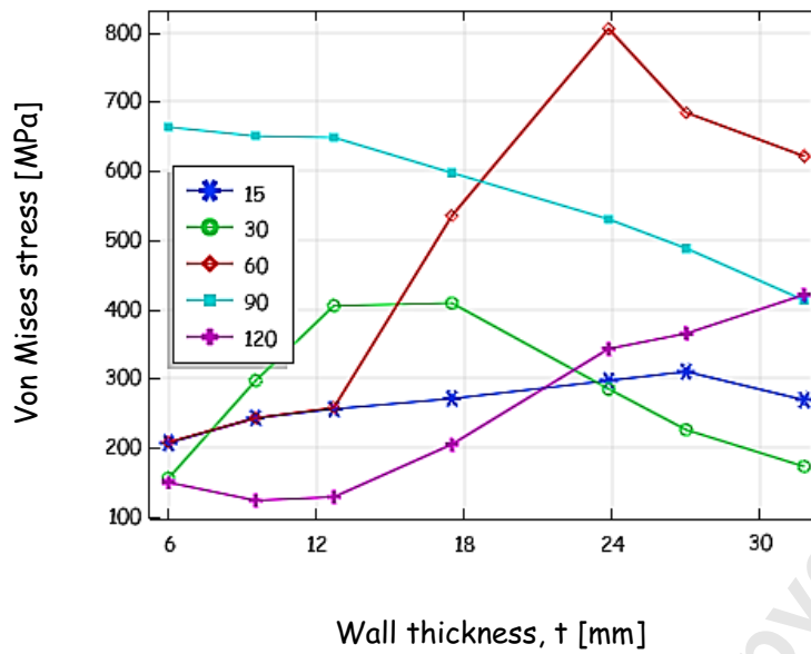
Figure 9. von Mises stress for buried pipeline damaged at invert for different spread angles
