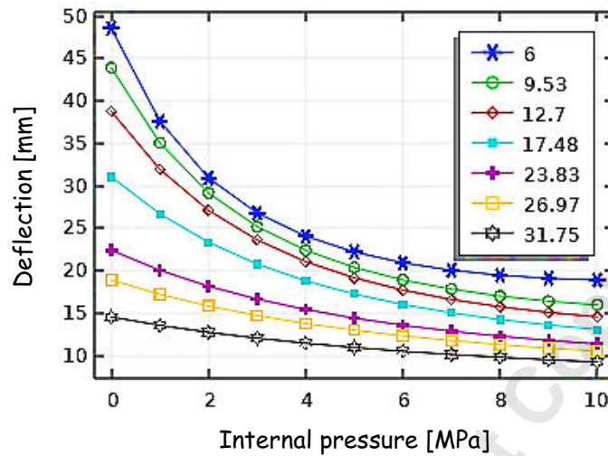
Figure 10. Deflection of intact pipeline under internal pressure
