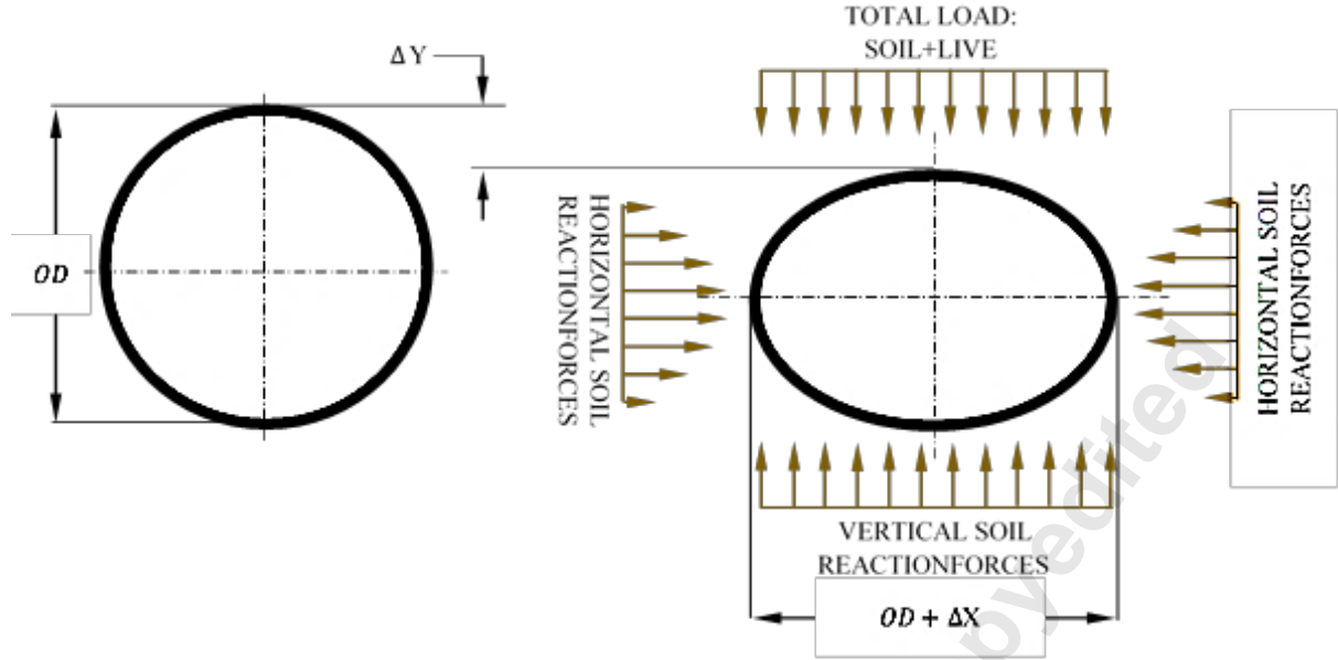
Figure 1. Theoretical Load Distribution in Buried Flexible Pipe Deflection.
