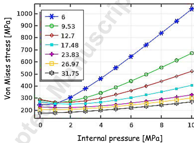
Figure 11. Von Mises stress of intact pipeline
