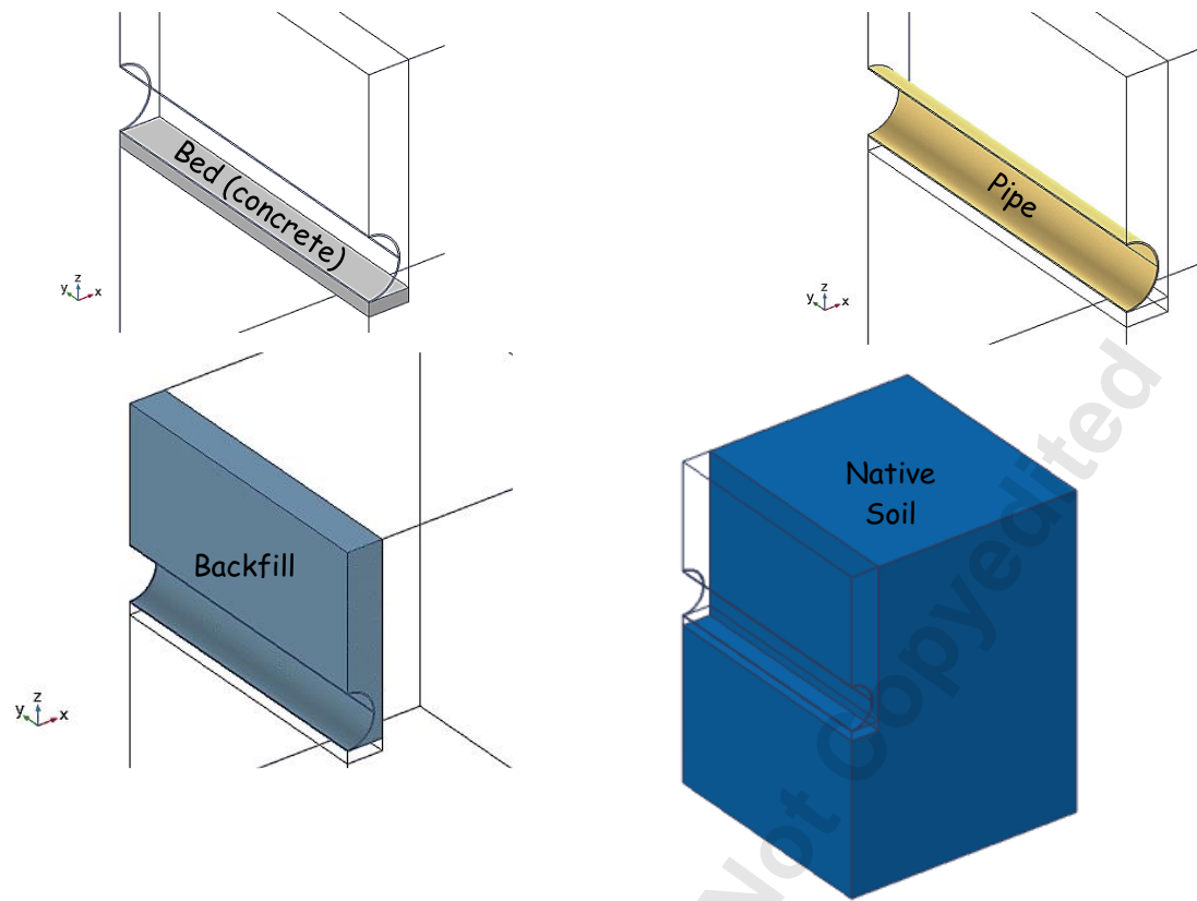
Figure 3. FE model with coupled domains
