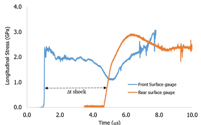
Fig. 6 Typical gauge trace for 10 mm thick copper impacting a 10.12-mm thick printed PLA at 567 m/s
