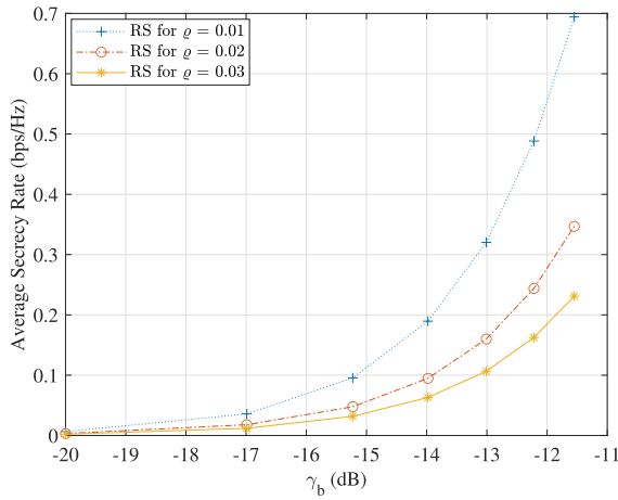
FIGURE 9. Impact of varying ( \varrho ) while evaluating average secrecy rate against desired SNR at \nu = 0.01 , \sigma = 0.1 , \mu = 0.01 .
