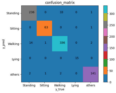
Fig. 6. Confusion matrix of pose behaviour classification model.
