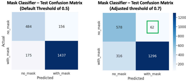
Fig. 7. BiT mask classifier final confusion matrix on the held-out test set.
