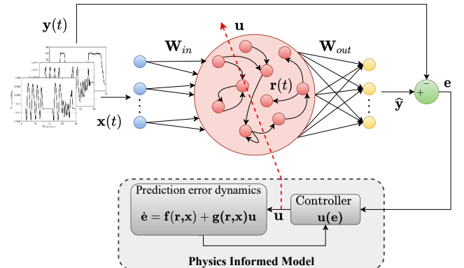
Fig. 2. Physics Informed Reservoir Computing Scheme
