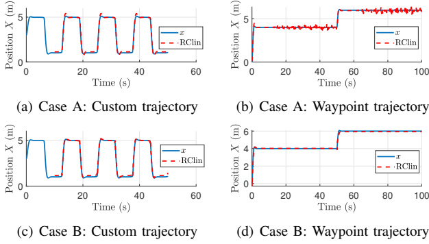
Fig. 9. Prediction results with/without control trajectories
