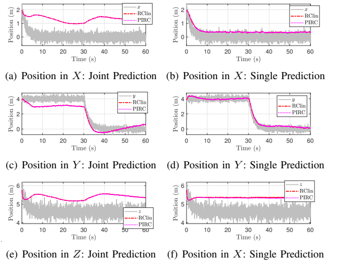
Fig. 5. Predictions of a random package delivery trajectory
