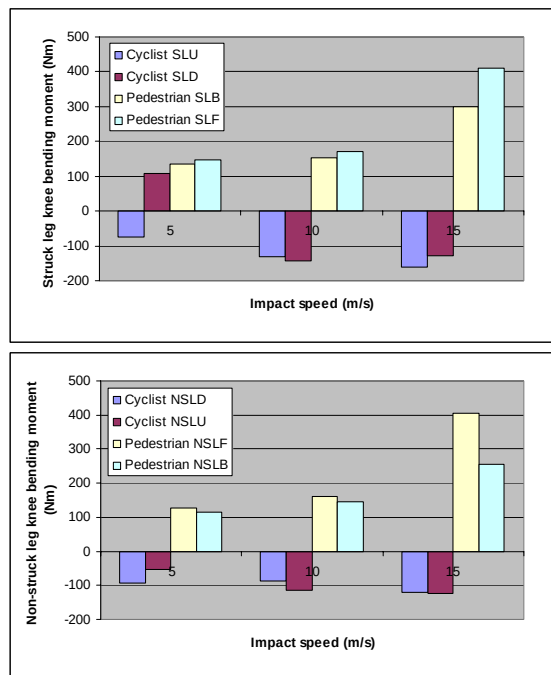
Figure 10. Knee bending moments for the struck and non-struck legs.
