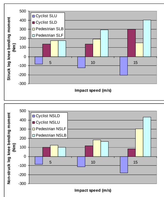
Figure 15. Knee bending moments for the struck and non-struck legs.
