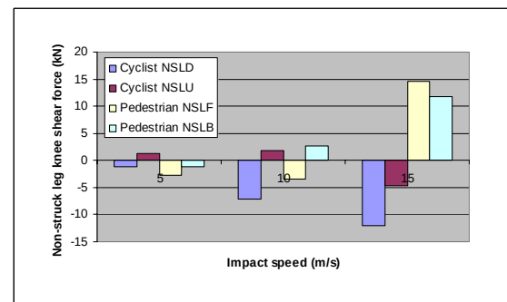
Figure 11. Knee shear forces for the struck and non-struck legs.
