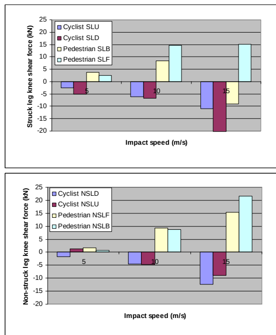
Figure 16. Knee shear forces for the struck and non-struck legs.
