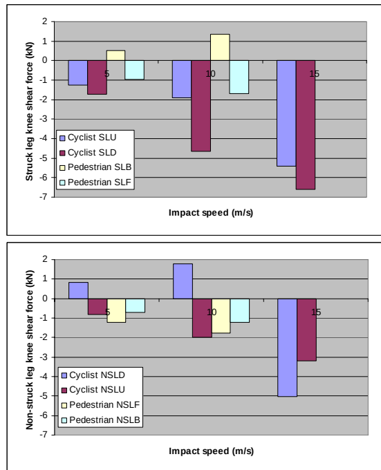
Figure 13. Knee shear forces for the struck and non-struck legs.
