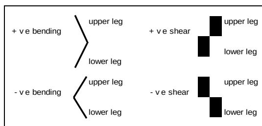
Figure 8. Sign convention for knee bending and shear.
