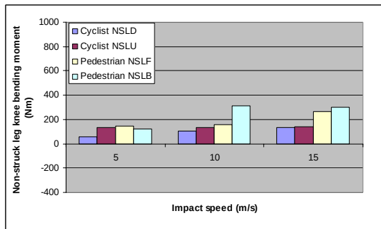
Figure 18: Knee bending moments for the struck and non-struck legs.
