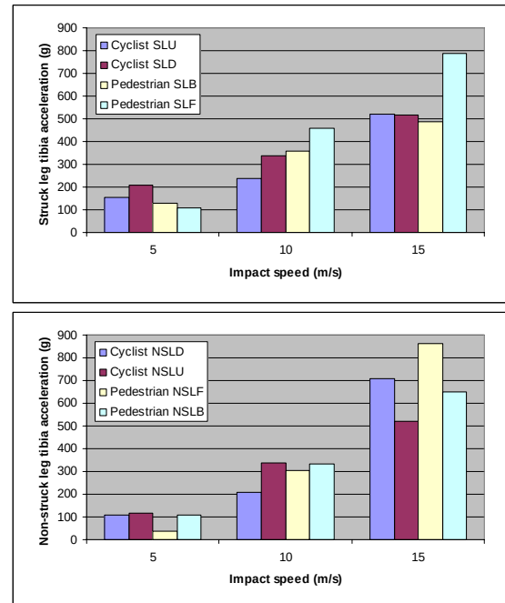
Figure 17: Tibia accelerations for the struck and non-struck legs.
