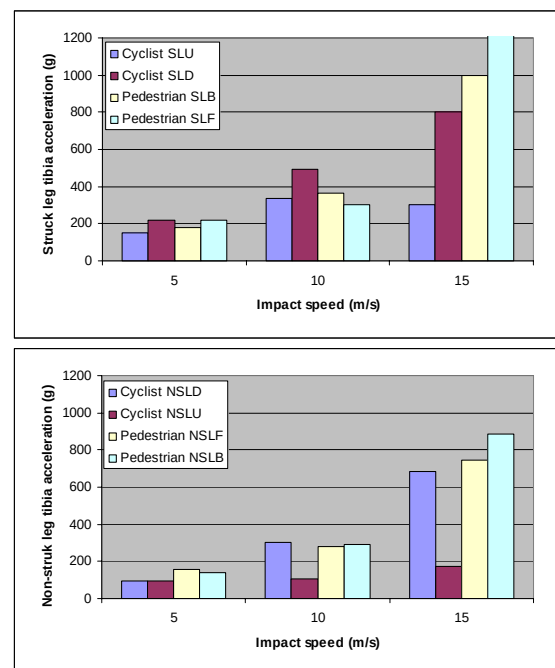
Figure 9. Tibia accelerations for the struck and non-struck legs.
