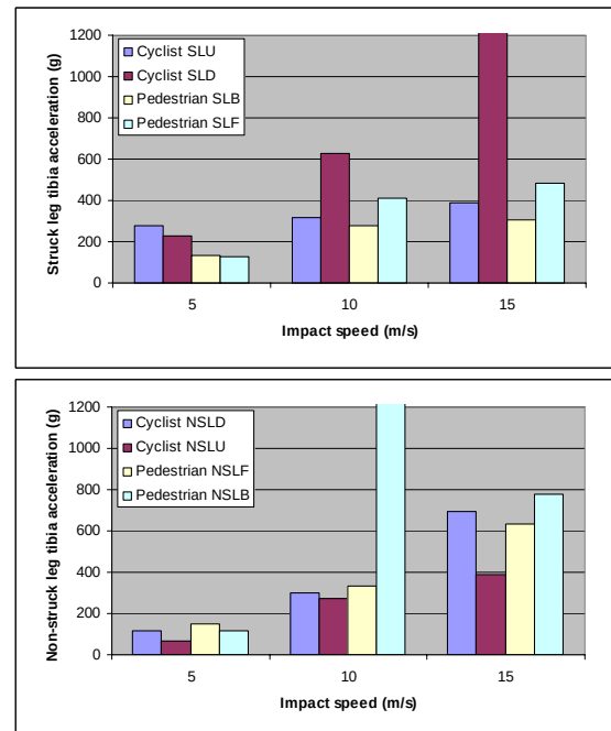
Figure 14: Tibia accelerations for the struck and non-struck legs
