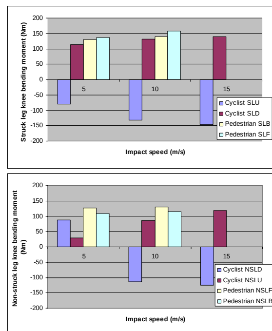
Figure 12. Knee bending moments for the struck and non-struck legs.
