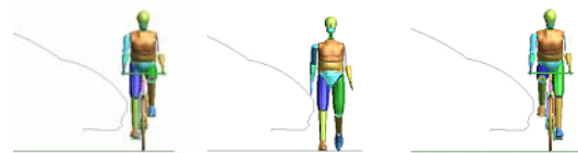
Figure 6. Cyclist and pedestrian leg positioning with respect to MPV front.
