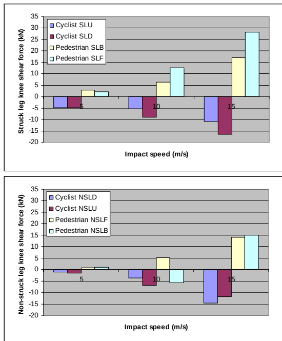
Figure 19. Knee shear forces for the struck and non-struck legs.
