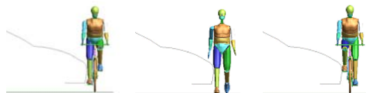
Figure 4. Cyclist and pedestrian leg positioning with respect to Supermini front.
