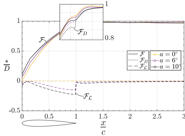
Fig. 5 Drag-normalised defect force, defect drag and defect lift component evolutions for a NACA0012 airfoil at Re_c = 1 \times 10^6 , M_\infty = 0.3 and \alpha = 0, 6, 10 .
