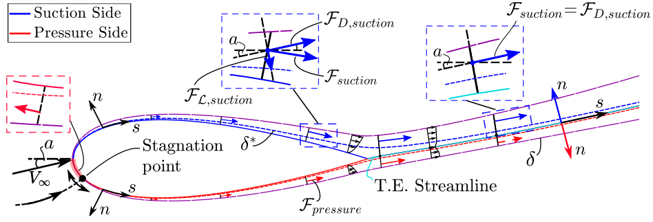
Fig. 3 Defect force definitions over an airfoil and the wake.
