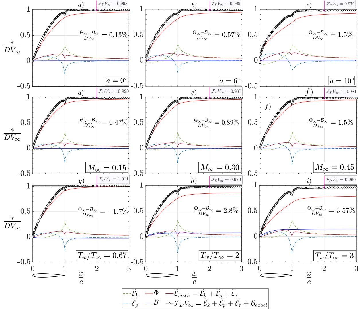
Fig. 13 Drag power-normalised viscous energy generation balance terms for a NACA0012 at fixed: a) - c) Re_c = 1 \times 10^6 , M_\infty = 0.3 d) - f) Re_c = 1 \times 10^7 , a = 4^\circ g) - i) Re_c = 1 \times 10^7 , M_\infty = 0.15 and a = 4^\circ .
