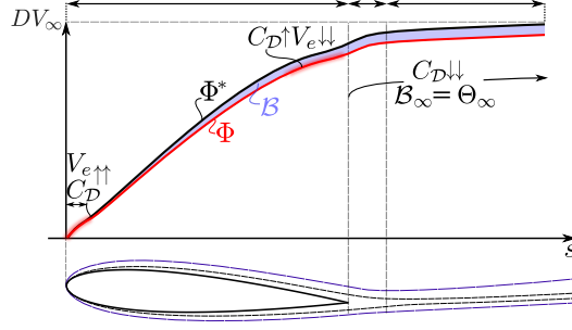
Fig. 7 Mechanical energy loss ( \Phi^* ) and viscous dissipation ( \Phi ) evolution for adiabatic compressible viscous flow. The deviation between the two trends is attributed to the additional baroclinic power imparted to the flow.
