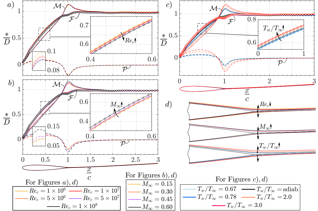
Fig. 6 Drag-normalised (suction + pressure side) defect force component evolutions for NACA0012 airfoil at constant \alpha = 4^\circ and various operating conditions.
