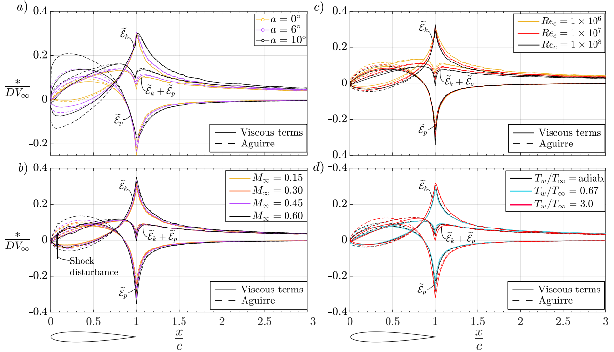
Fig. 14 Comparison of viscous mechanical energy generation flux components against Aguirre's [36] velocity decomposition method for a NACA0012 airfoil at fixed: a) Re_c = 1 \times 10^6 , M_\infty = 0.3 b) Re_c = 1 \times 10^7 , a = 4^\circ c) M_\infty = 0.3 a = 4^\circ d) Re_c = 1 \times 10^7 , M_\infty = 0.15 , a = 4^\circ .
