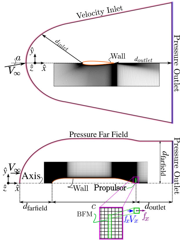
Fig. A1 2D CFD domain of NACA 0012 airfoil (upper) and 2D axisymmetric domain of fuselage - BLI propulsor assembly (lower) with annotated geometric features, boundary conditions and partial mesh sample.
