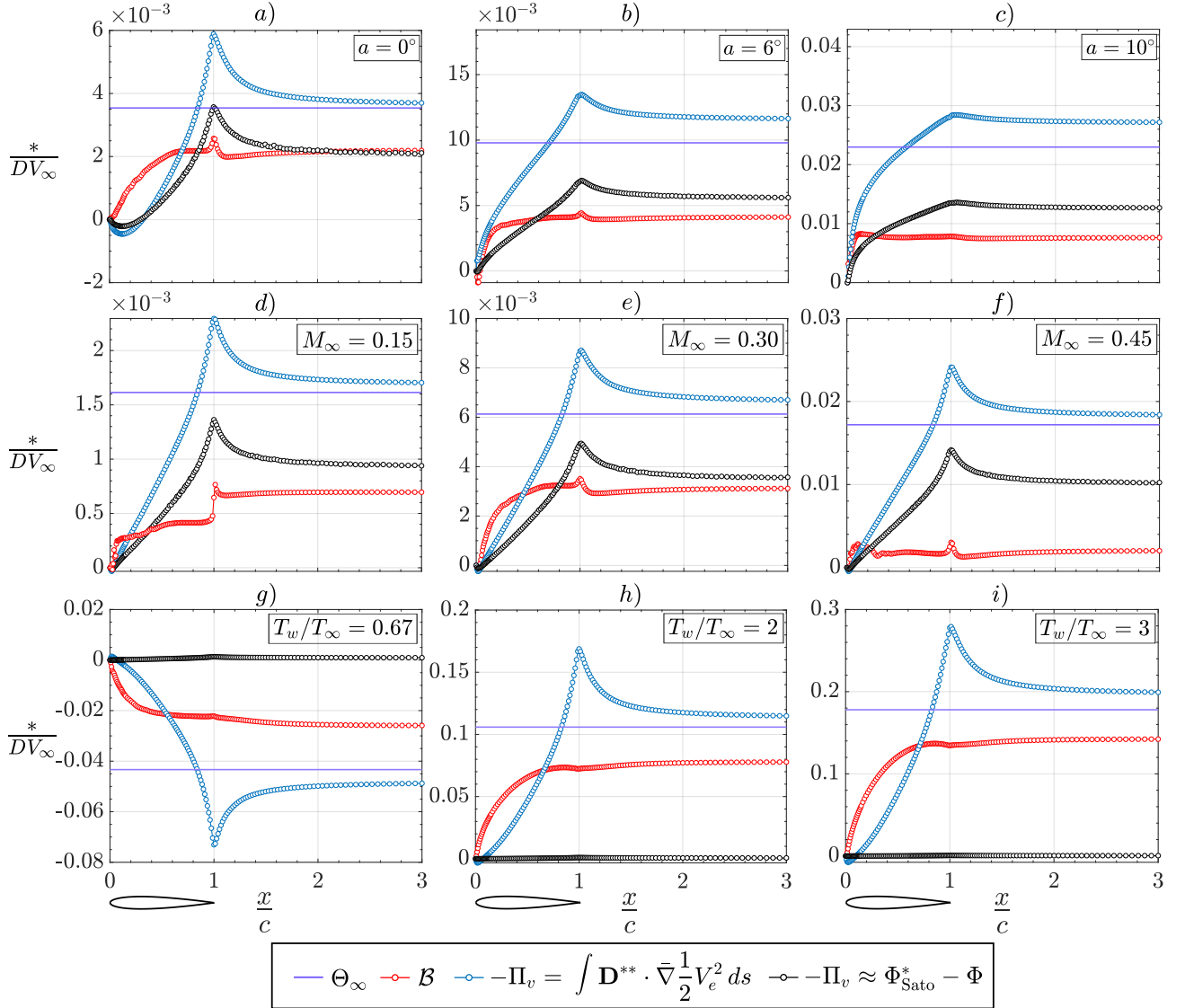
Fig. 11 Residual baroclinic power expression comparison for a NACA0012 at fixed: a) - c) Re_c = 1 \times 10^6 , M_\infty = 0.3 . d) - f) Re_c = 1 \times 10^7 , a = 4^\circ g) - i) Re_c = 1 \times 10^7 , M_\infty = 0.15 , a = 4^\circ .
