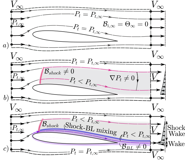
Fig. E1 Illustration of shock-induced baroclinic losses for a 2-D airfoil: a) Inviscid, subsonic flow. b) Inviscid, transonic flow with shock. c) Transonic viscous flow with shock.
