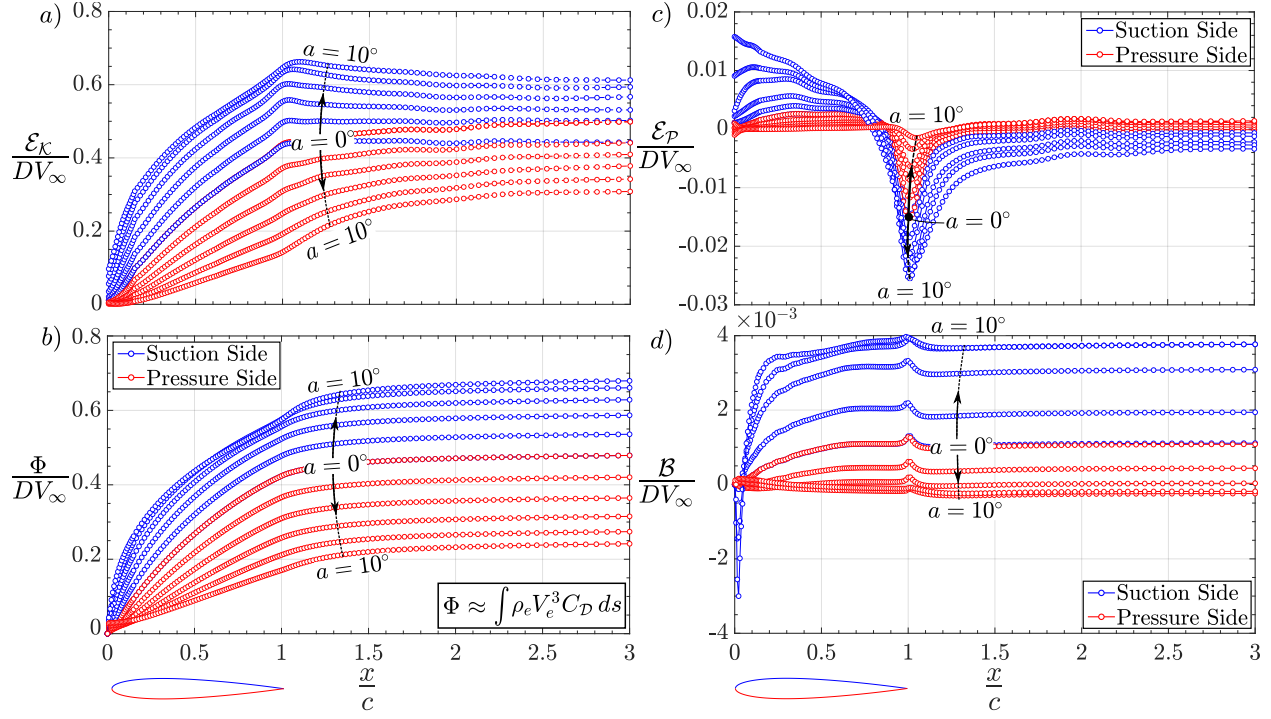
Fig. 8 Evolution of drag power-normalised defect mechanical energy components for NACA0012 airfoil suction and pressure surfaces at Re_c = 1 \times 10^6 , M_\infty = 0.3 and a = 0^\circ, 2^\circ, 4^\circ, 6^\circ, 8^\circ, 10^\circ .
