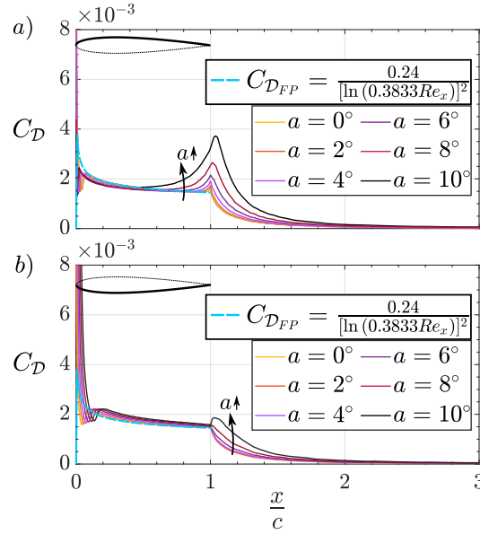
Fig. 9 C_D evolution of a NACA0012 airfoil at Re_c = 1 \times 10^6 , M_\infty = 0.3 and a = 0^\circ, 2^\circ, 4^\circ, 6^\circ, 8^\circ, 10^\circ : a) Suction Side b) Pressure Side. The cyan curves show the C_{D_{FP}} expression for a smooth turbulent flat plate by Sato [26].
