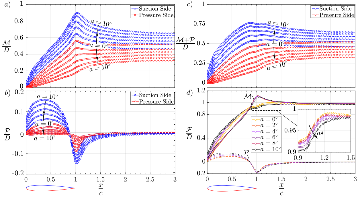
Fig. 4 Drag-normalised defect force component evolutions for NACA0012 airfoil at Re_c = 1 \times 10^6 , M_\infty = 0.3 and \alpha = 0, 2, 4, 6, 8, 10 : a) - c) Individual evolutions from suction and pressure sides. d) Total (pressure + suction side) defect force components.
