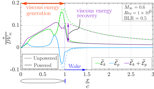
Fig. 15 Drag power-normalised viscous energy flux terms for an unpowered (dashed) and a BLI powered (solid) fuselage at Re_c = 1 \times 10^6 and M_\infty = 0.6 .
