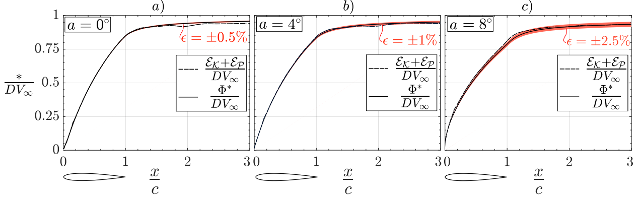
Fig. 10 Drag power-normalised mechanical loss evolution of a NACA0012 at Re_c = 1 \times 10^6 , M_\infty = 0.3 and varying a , as obtained from \mathcal{E}_K + \mathcal{E}_P and \Phi^* .
