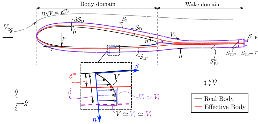
Fig. 1 Superpositioned real viscous flow and equivalent inviscid flow fields over the real and effective (inviscid) aerodynamic bodies, along with annotated control volume definitions and relevant flow features.
