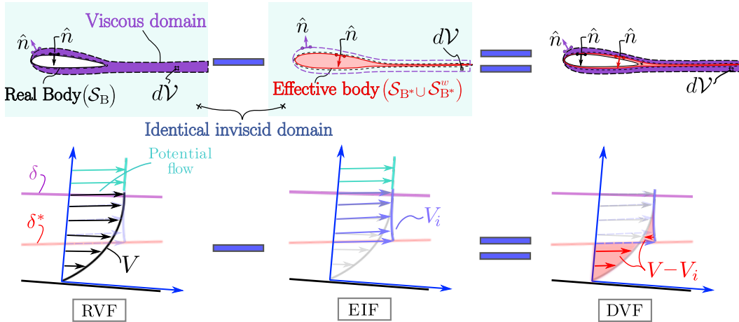
Fig. 2 RVF, EIF and DVF control volume definitions (upper) and corresponding velocity profiles (lower).
