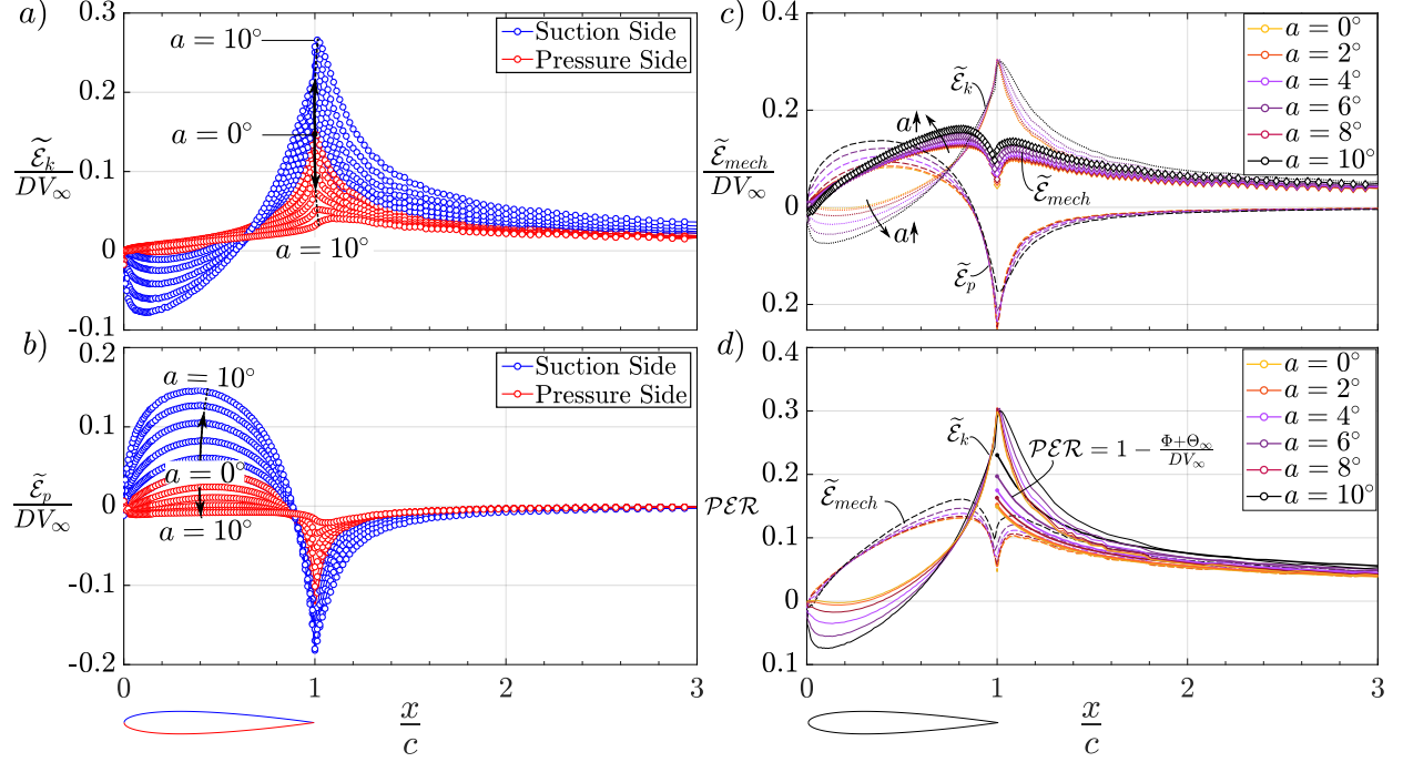
Fig. 12 Drag power-normalised viscous mechanical energy generation components for NACA0012 airfoil at Re_c = 1 \times 10^6 , M_\infty = 0.3 and varying a .
