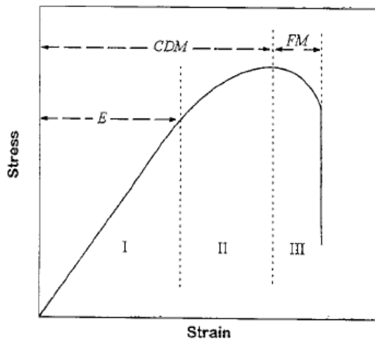
FIGURE 1: On its way to failure a 'quasi-brittle' solid (not just bone) exhibits a stress/ strain behaviour, which can be split in three major domains: the elastic range (E), the continuum damage mechanics range (CDM), and the fracture mechanics (FM) one. In phase-II some of the input energy goes to increase the elastic strain energy of the body and some is dissipated in the generation of tiny cracks. In phase-III the product of d\sigma^*d\varepsilon (increments of stress and strain) is negative and the ability of the material to increase its strength is rapidly counterbalanced by the reduction in the effective cross sectional area caused by the growth of a major crack. Mechanical tests for toughness are designed to take advantage of and enhance the effects of each phase. Depending on the kind and combination of applied stresses, the geometry of the specimen (which determines the stress field) and perhaps some specialised material properties (anisotropy, regional heterogeneity) the relative length of the three regions can vary widely and at will by the experienced experimenter who aims to isolate one or the other kind of behaviour.
