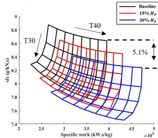
Figure 6 - Turboprop cycle design space without efficiency correction
