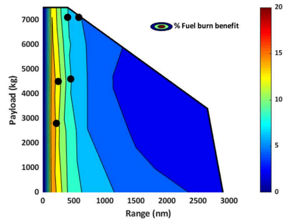
Figure 24 - Overall fuel burn benefit, regional turboprop, Scenario 2
