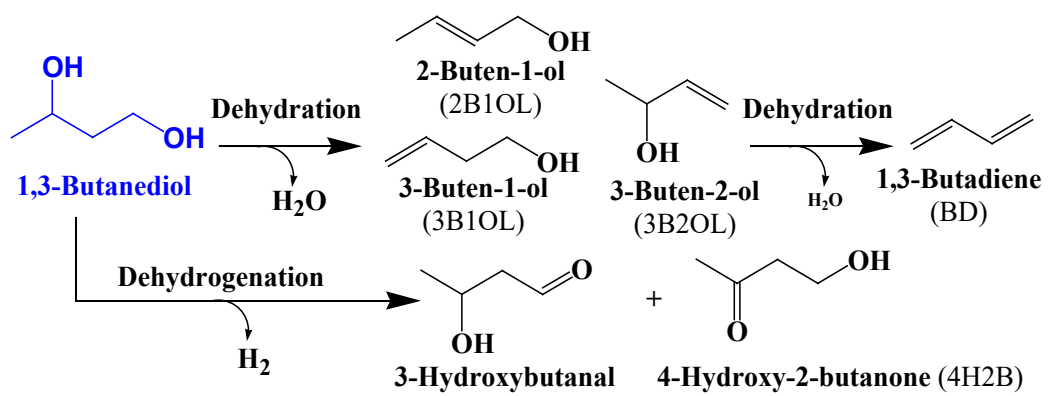
Fig. 7. 1,3-BDO derivatives.
