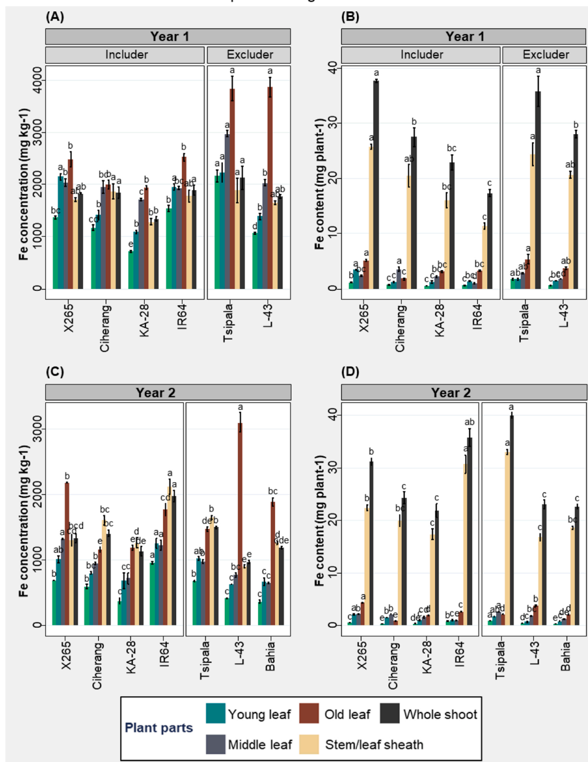
Fig. 4. Iron concentrations and contents in above-ground tissues at flowering stage. Data are means \pm standard errors ( n = 4 ). Common letters indicate no significant difference between genotypes for a given tissue by Tukey's HSD test.
