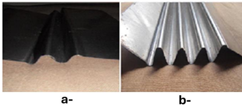
Fig. 17. First stage of the formed profile consisting of two waves (a) and second stage of the formed profile consisting of four waves (b)
