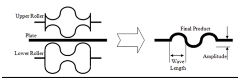
Fig. 1. Production of a corrugated plate characterised by amplitude and wavelength
