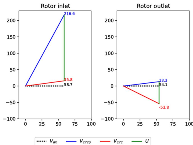
Fig. 12 Rotor velocity triangle at peak power production N:40% in baseline contra-rotating turbine mode. Velocity units in m/s. Positive values in direction of rotation.
