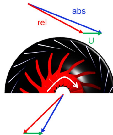
Fig. 12 Rotor velocity triangle at peak power production N:40% in baseline contra-rotating turbine mode. Velocity units in m/s. Positive values in direction of rotation.
