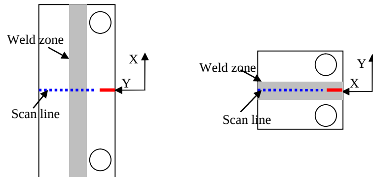
Fig.3 ESE(T) and C(T) samples
