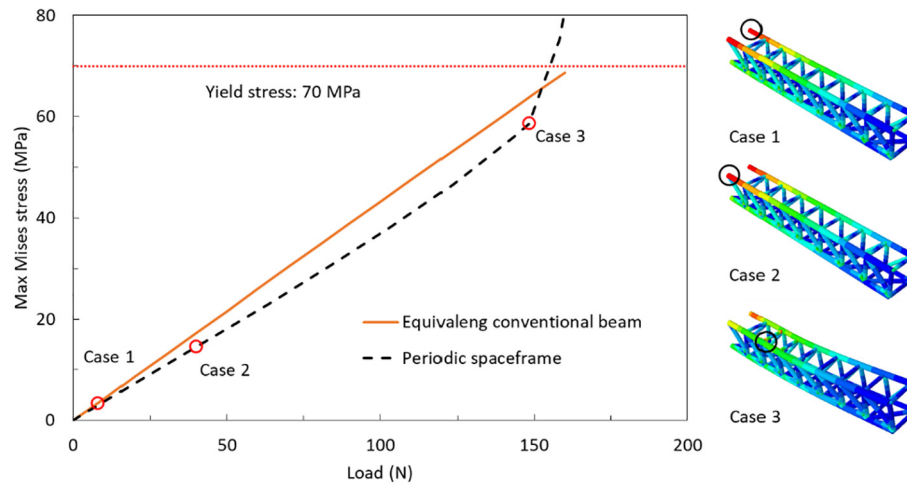
Fig. 8. Maximum stress in the periodic spaceframe and equivalent conventional beam structures as a function of the applied load, highlighting the enhanced performance of the periodic spaceframe.
